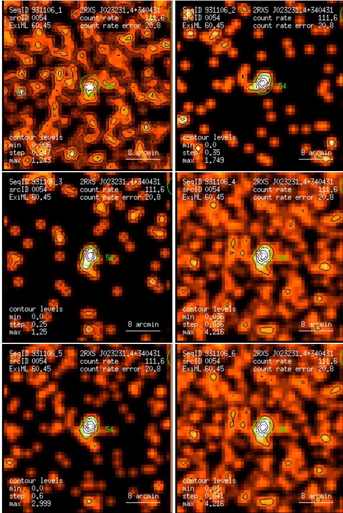
Figure 54: RASS 931106: detection 0054: band rate images, Gaussian filter: (1) PSPC channels 11 – 41, (2) 52 – 90, (3) 91 – 201, (4) 11 – 235, (5) 52 – 201, (6) 11 – 201. Broad band rates in counts/ks. Band rate contour levels in counts/ks/arcmin 2 .
