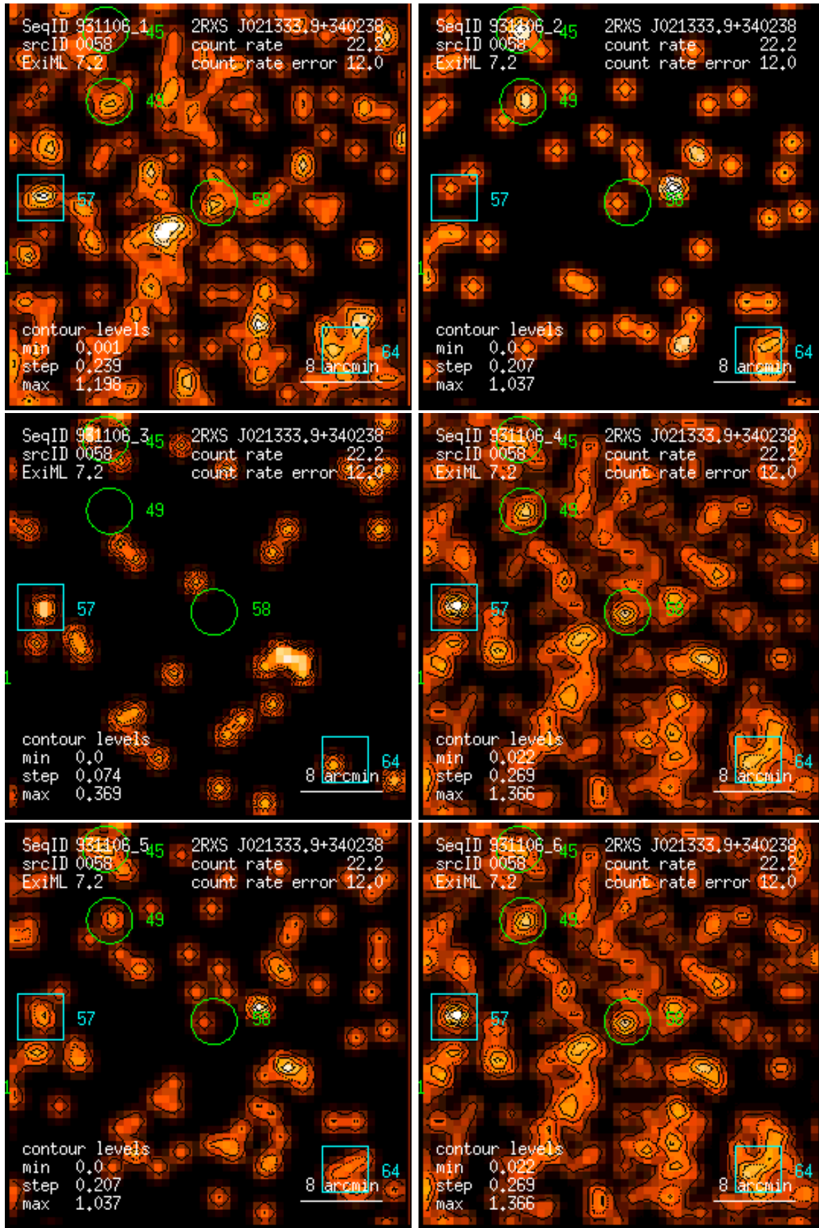
Figure 58: RASS 931106: detection 0058: band rate images, Gaussian filter: (1) PSPC channels 11 – 41, (2) 52 – 90, (3) 91 – 201, (4) 11 – 235, (5) 52 – 201, (6) 11 – 201. Broad band rates in counts/ks. Band rate contour levels in counts/ks/arcmin 2 .
