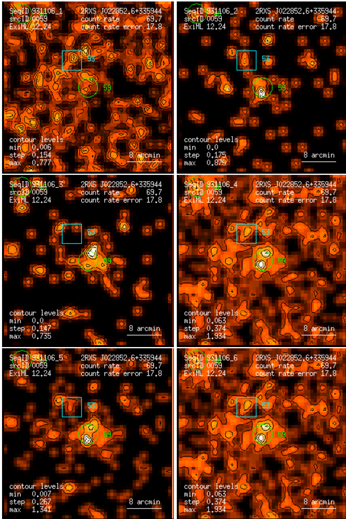
Figure 59: RASS 931106: detection 0059: band rate images, Gaussian filter: (1) PSPC channels 11 – 41, (2) 52 – 90, (3) 91 – 201, (4) 11 – 235, (5) 52 – 201, (6) 11 – 201. Broad band rates in counts/ks. Band rate contour levels in counts/ks/arcmin 2 .
