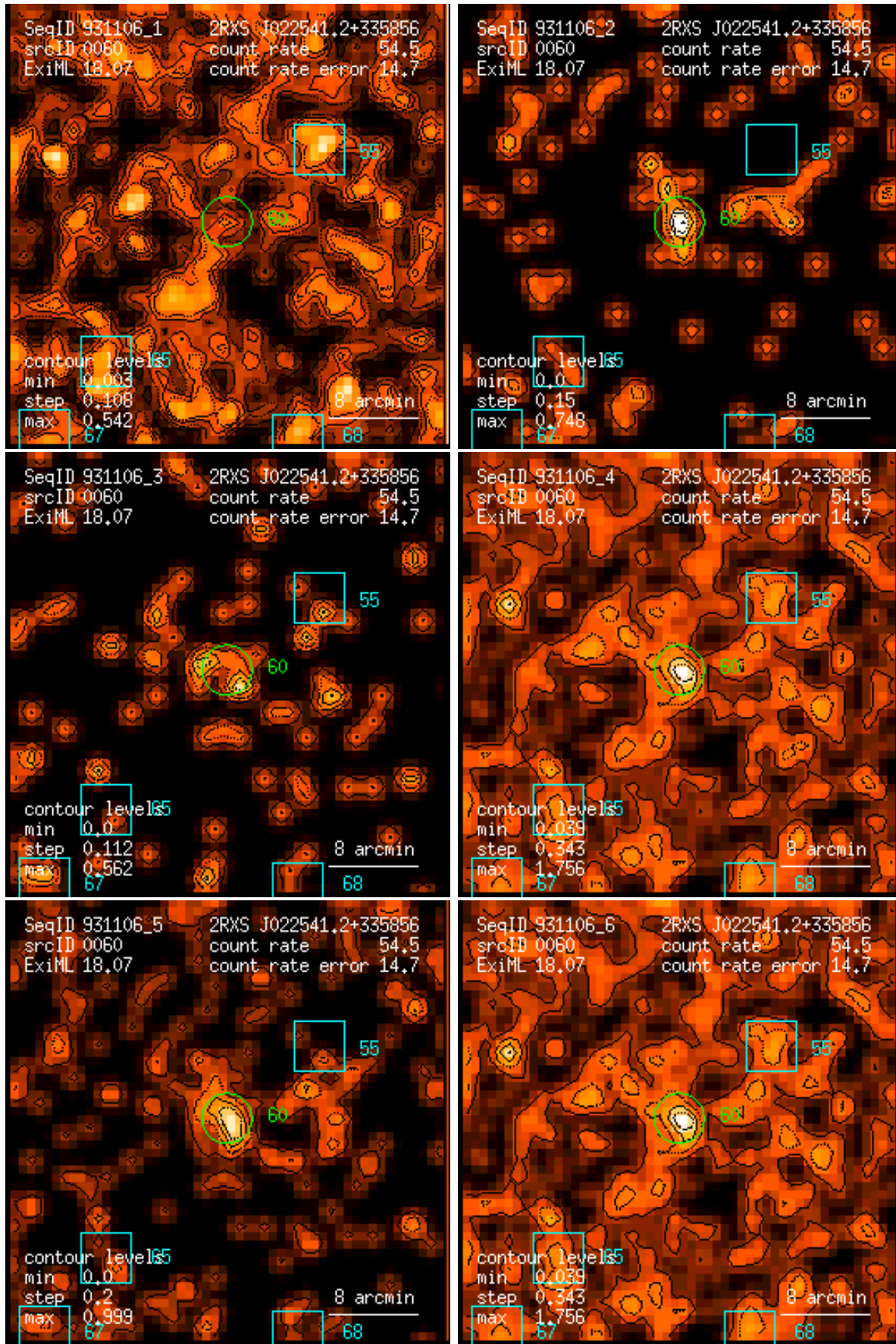
Figure 60: RASS 931106: detection 0060: band rate images, Gaussian filter: (1) PSPC channels 11 – 41, (2) 52 – 90, (3) 91 – 201, (4) 11 – 235, (5) 52 – 201, (6) 11 – 201. Broad band rates in counts/ks. Band rate contour levels in counts/ks/arcmin 2 .
