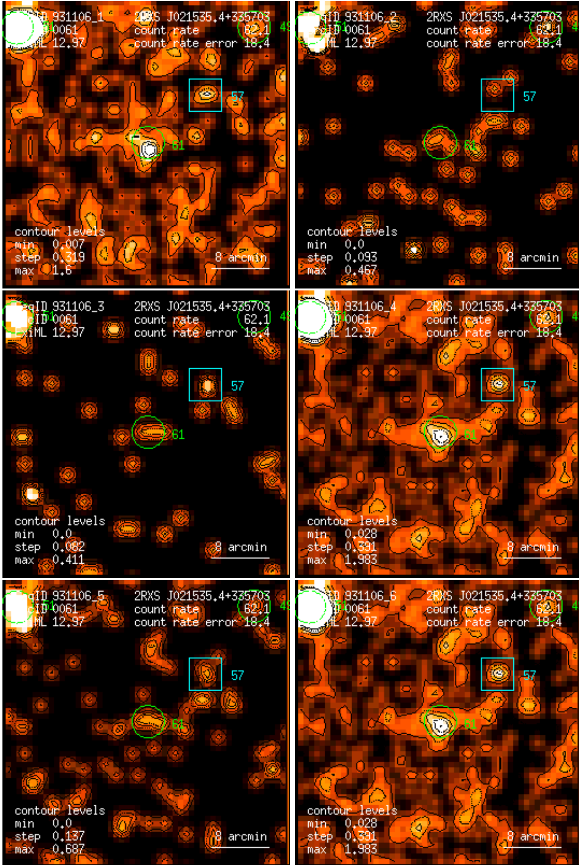
Figure 61: RASS 931106: detection 0061: band rate images, Gaussian filter: (1) PSPC channels 11 – 41, (2) 52 – 90, (3) 91 – 201, (4) 11 – 235, (5) 52 – 201, (6) 11 – 201. Broad band rates in counts/ks. Band rate contour levels in counts/ks/arcmin 2 .
