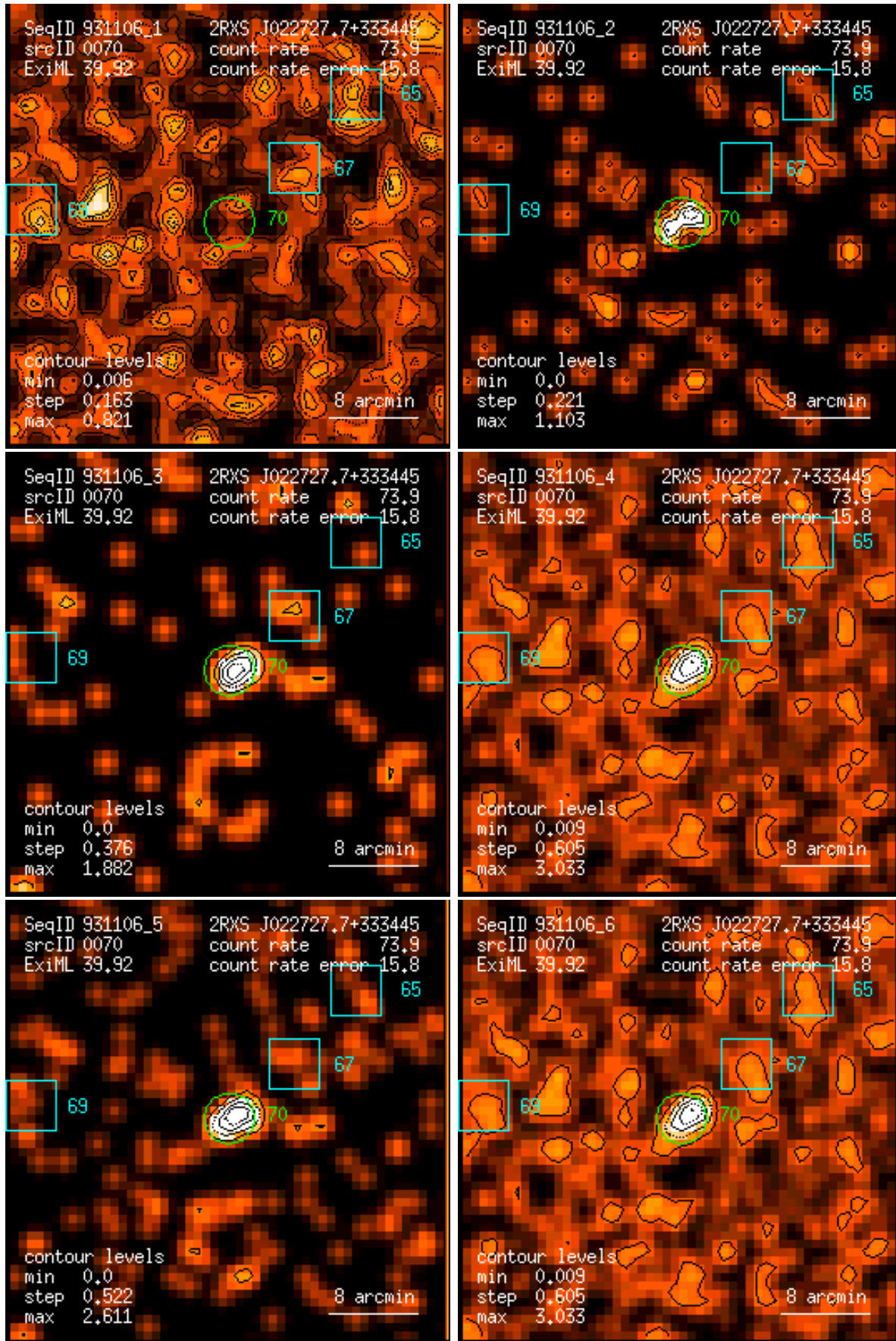
Figure 70: RASS 931106: detection 0070: band rate images, Gaussian filter: (1) PSPC channels 11 – 41, (2) 52 – 90, (3) 91 – 201, (4) 11 – 235, (5) 52 – 201, (6) 11 – 201. Broad band rates in counts/ks. Band rate contour levels in counts/ks/arcmin 2 .
