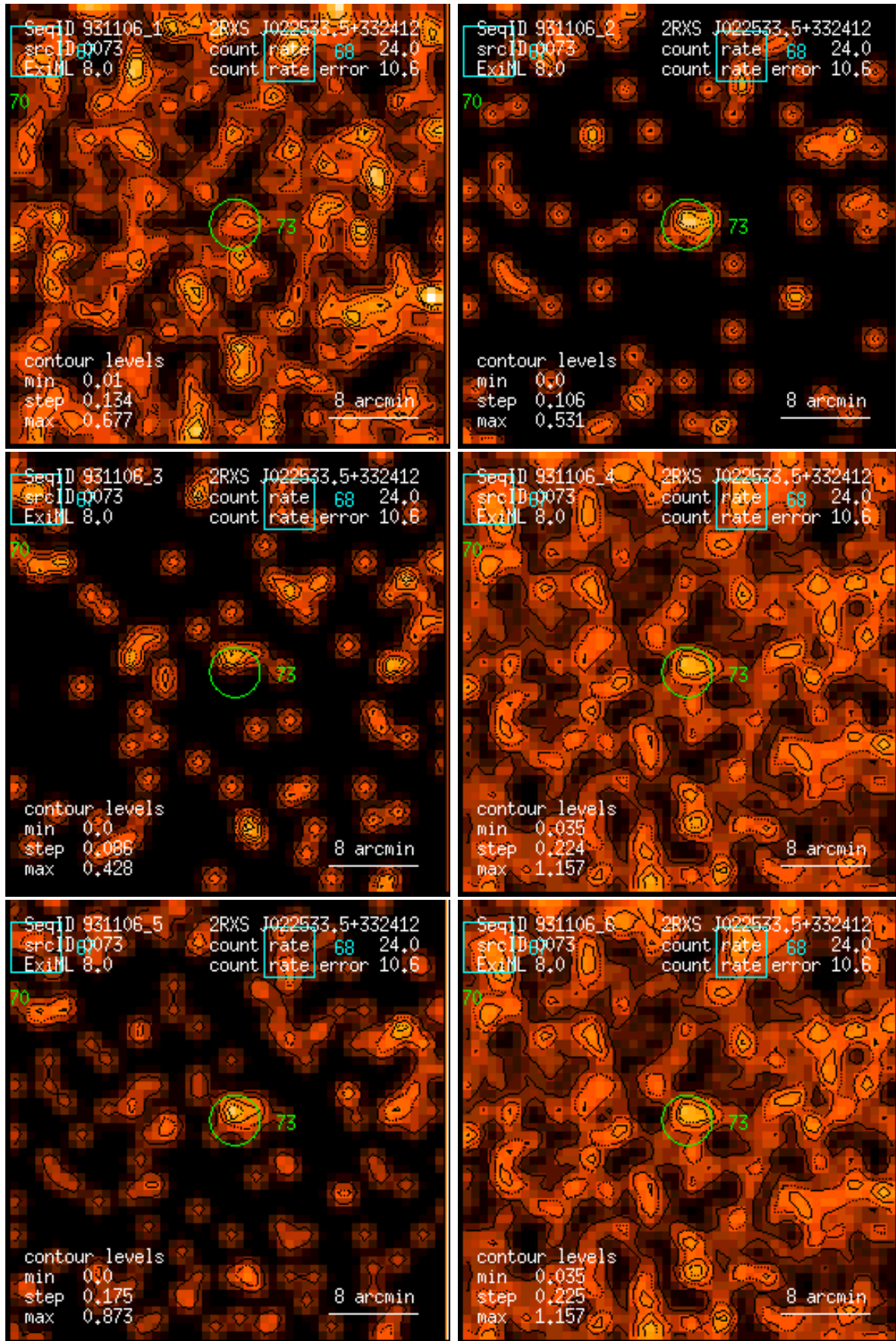
Figure 73: RASS 931106: detection 0073: band rate images, Gaussian filter: (1) PSPC channels 11 – 41, (2) 52 – 90, (3) 91 – 201, (4) 11 – 235, (5) 52 – 201, (6) 11 – 201. Broad band rates in counts/ks. Band rate contour levels in counts/ks/arcmin 2 .
