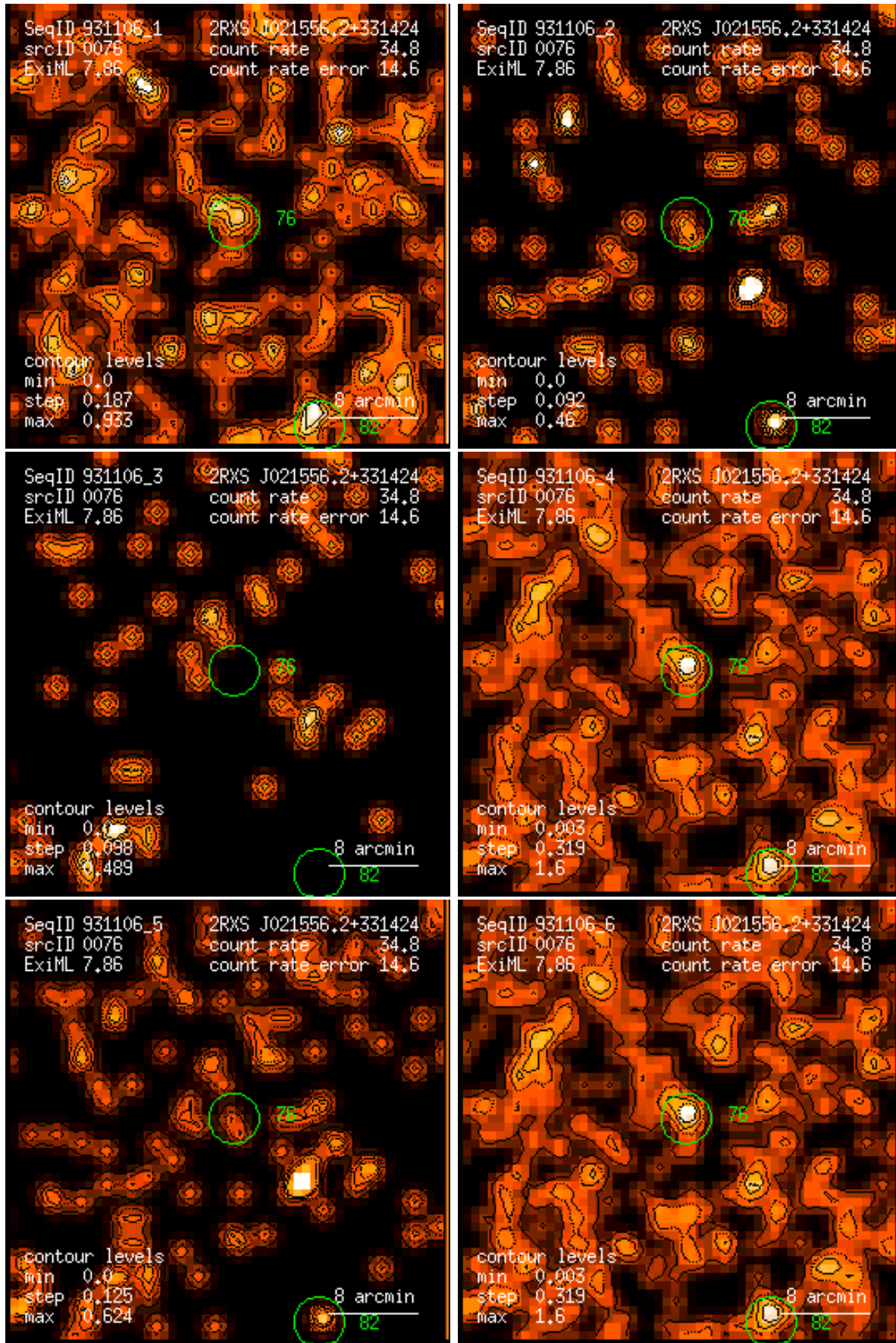
Figure 76: RASS 931106: detection 0076: band rate images, Gaussian filter: (1) PSPC channels 11 – 41, (2) 52 – 90, (3) 91 – 201, (4) 11 – 235, (5) 52 – 201, (6) 11 – 201. Broad band rates in counts/ks. Band rate contour levels in counts/ks/arcmin 2 .
