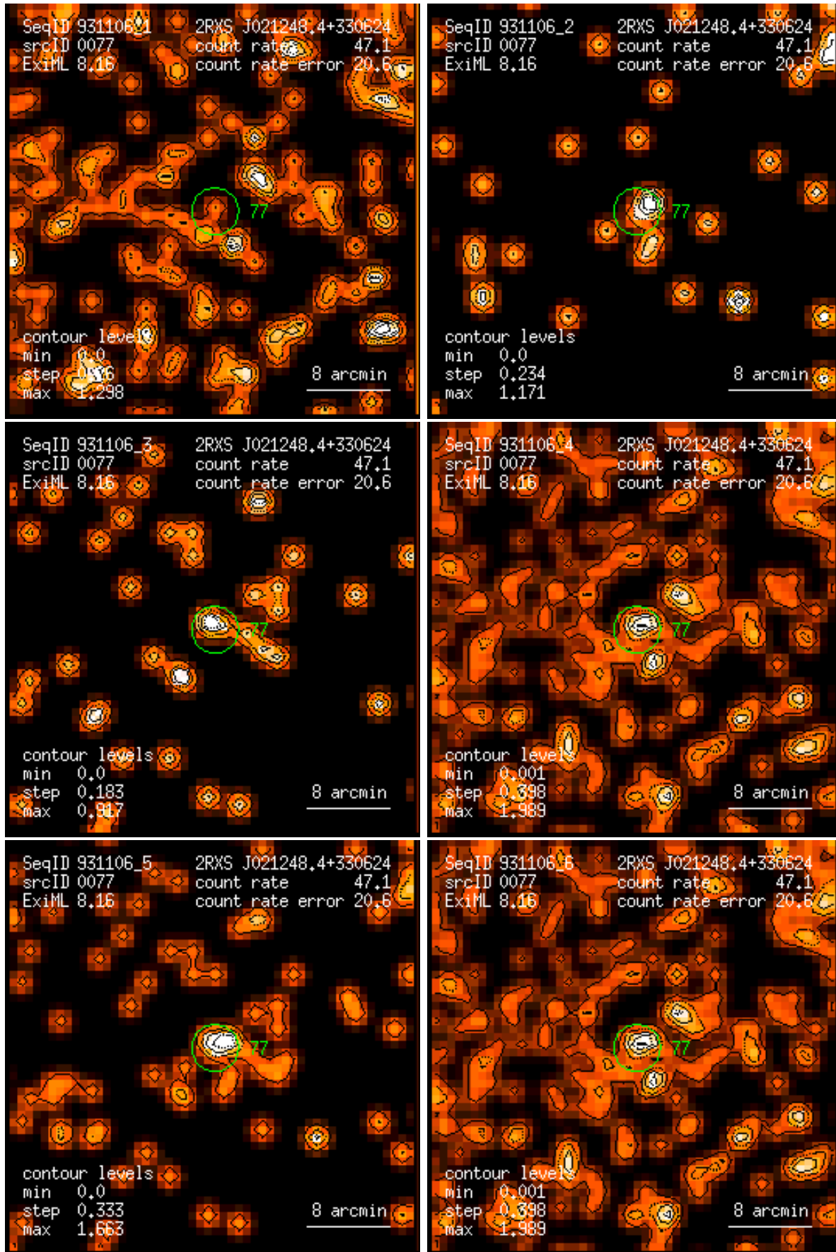
Figure 77: RASS 931106: detection 0077: band rate images, Gaussian filter: (1) PSPC channels 11 – 41, (2) 52 – 90, (3) 91 – 201, (4) 11 – 235, (5) 52 – 201, (6) 11 – 201. Broad band rates in counts/ks. Band rate contour levels in counts/ks/arcmin 2 .
