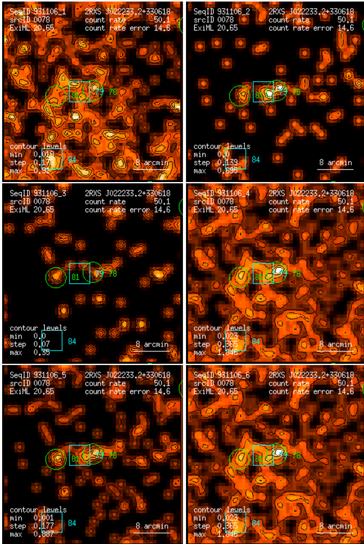
Figure 78: RASS 931106: detection 0078: band rate images, Gaussian filter: (1) PSPC channels 11 – 41, (2) 52 – 90, (3) 91 – 201, (4) 11 – 235, (5) 52 – 201, (6) 11 – 201. Broad band rates in counts/ks. Band rate contour levels in counts/ks/arcmin 2 .
