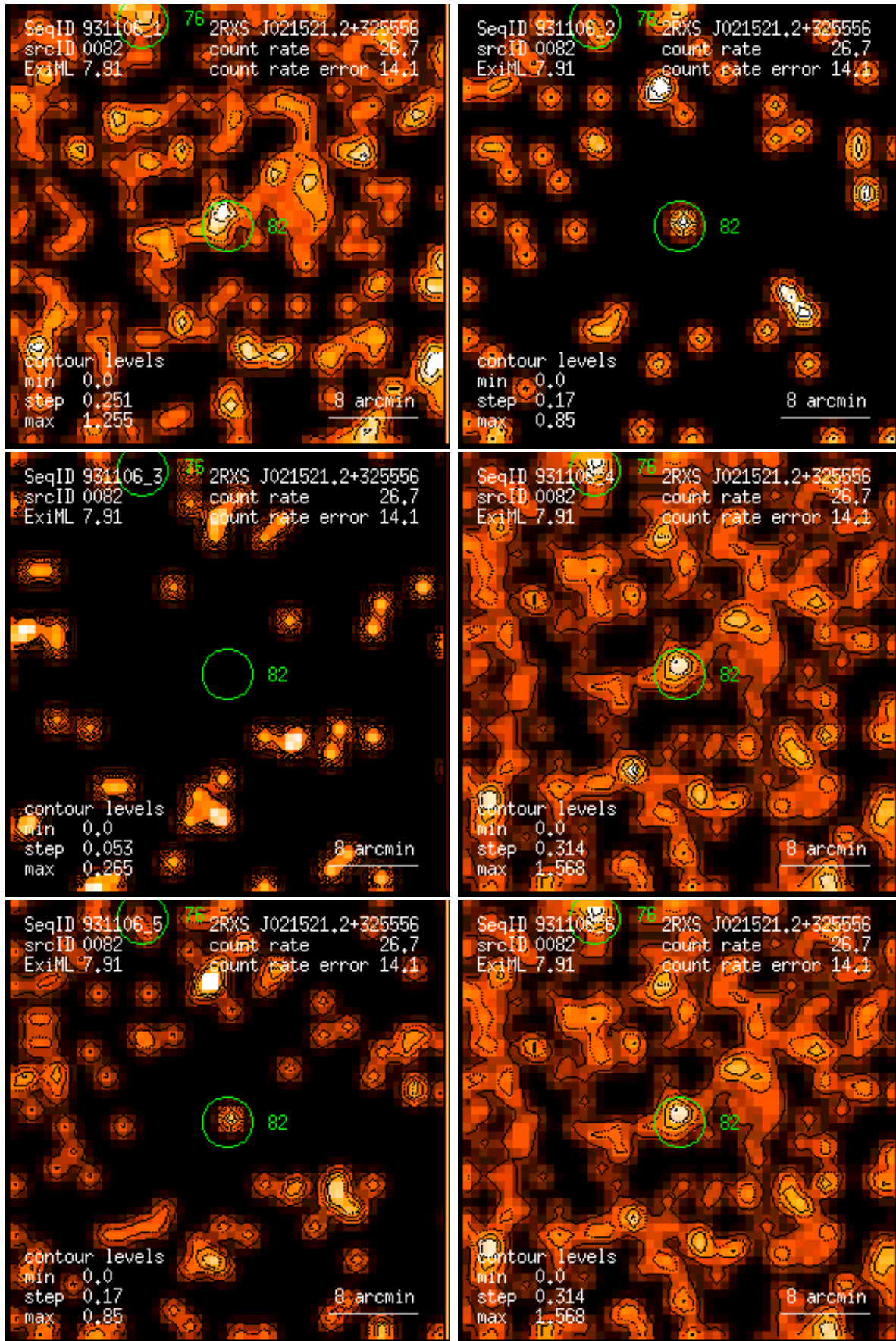
Figure 82: RASS 931106: detection 0082: band rate images, Gaussian filter: (1) PSPC channels 11 – 41, (2) 52 – 90, (3) 91 – 201, (4) 11 – 235, (5) 52 – 201, (6) 11 – 201. Broad band rates in counts/ks. Band rate contour levels in counts/ks/arcmin 2 .
