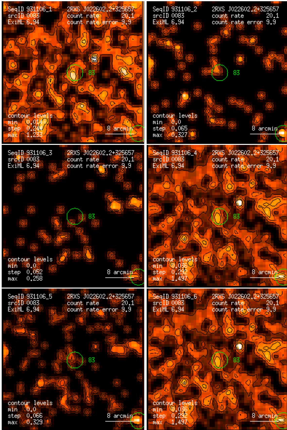
Figure 83: RASS 931106: detection 0083: band rate images, Gaussian filter: (1) PSPC channels 11 – 41, (2) 52 – 90, (3) 91 – 201, (4) 11 – 235, (5) 52 – 201, (6) 11 – 201. Broad band rates in counts/ks. Band rate contour levels in counts/ks/arcmin 2 .
