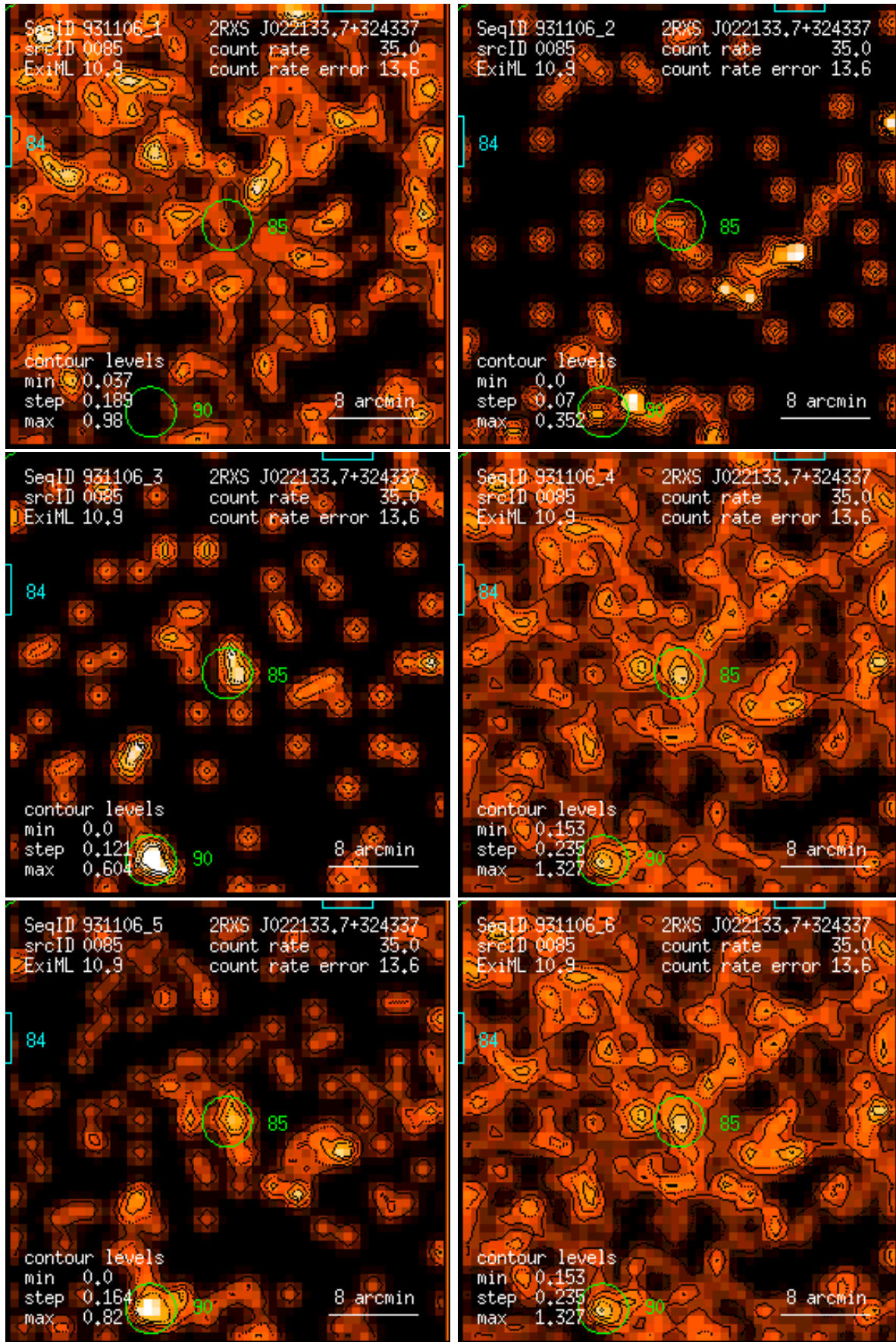
Figure 85: RASS 931106: detection 0085: band rate images, Gaussian filter: (1) PSPC channels 11 – 41, (2) 52 – 90, (3) 91 – 201, (4) 11 – 235, (5) 52 – 201, (6) 11 – 201. Broad band rates in counts/ks. Band rate contour levels in counts/ks/arcmin 2 .
