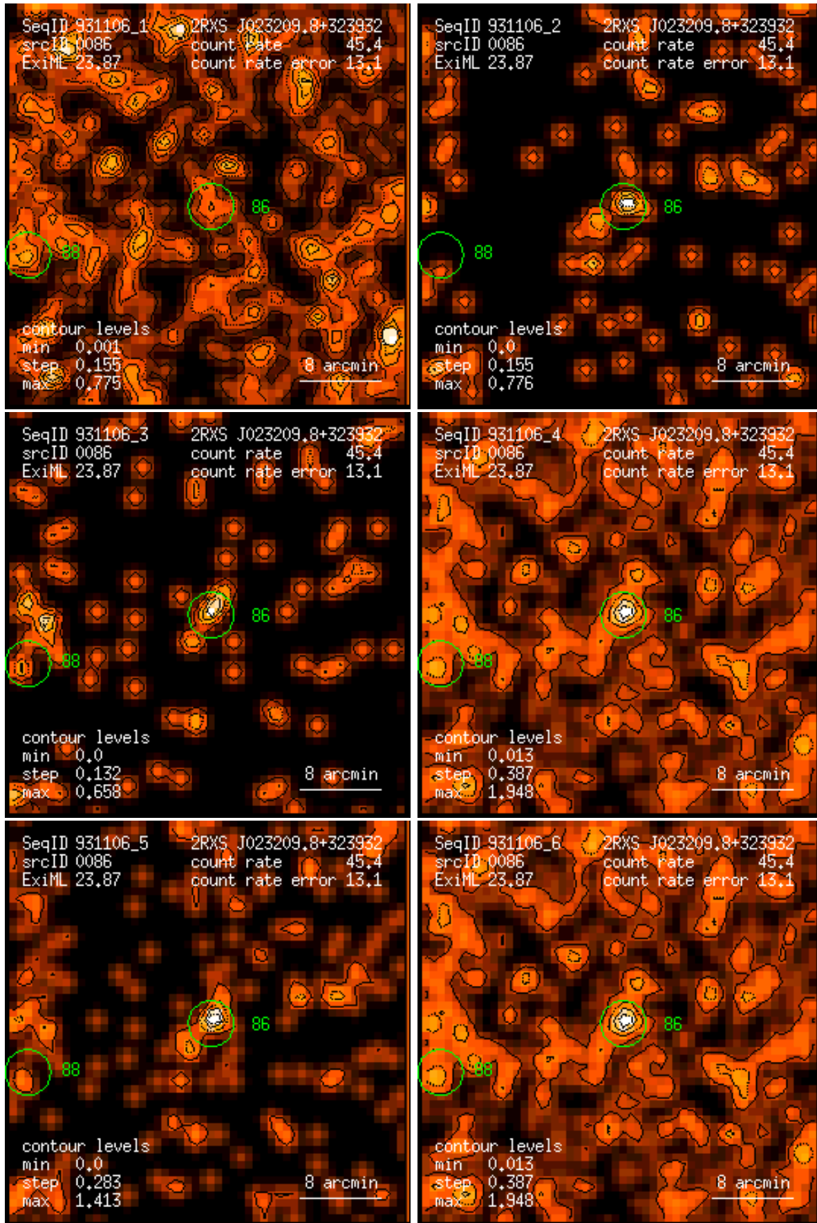
Figure 86: RASS 931106: detection 0086: band rate images, Gaussian filter: (1) PSPC channels 11 – 41, (2) 52 – 90, (3) 91 – 201, (4) 11 – 235, (5) 52 – 201, (6) 11 – 201. Broad band rates in counts/ks. Band rate contour levels in counts/ks/arcmin 2 .
