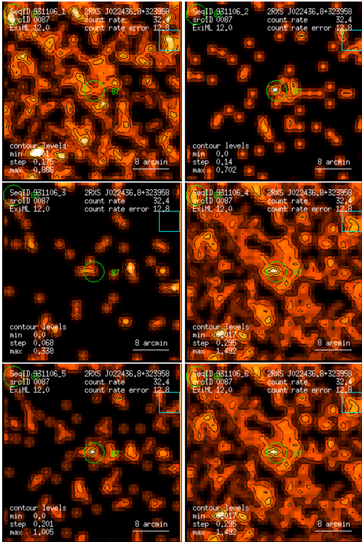
Figure 87: RASS 931106: detection 0087: band rate images, Gaussian filter: (1) PSPC channels 11 – 41, (2) 52 – 90, (3) 91 – 201, (4) 11 – 235, (5) 52 – 201, (6) 11 – 201. Broad band rates in counts/ks. Band rate contour levels in counts/ks/arcmin 2 .
