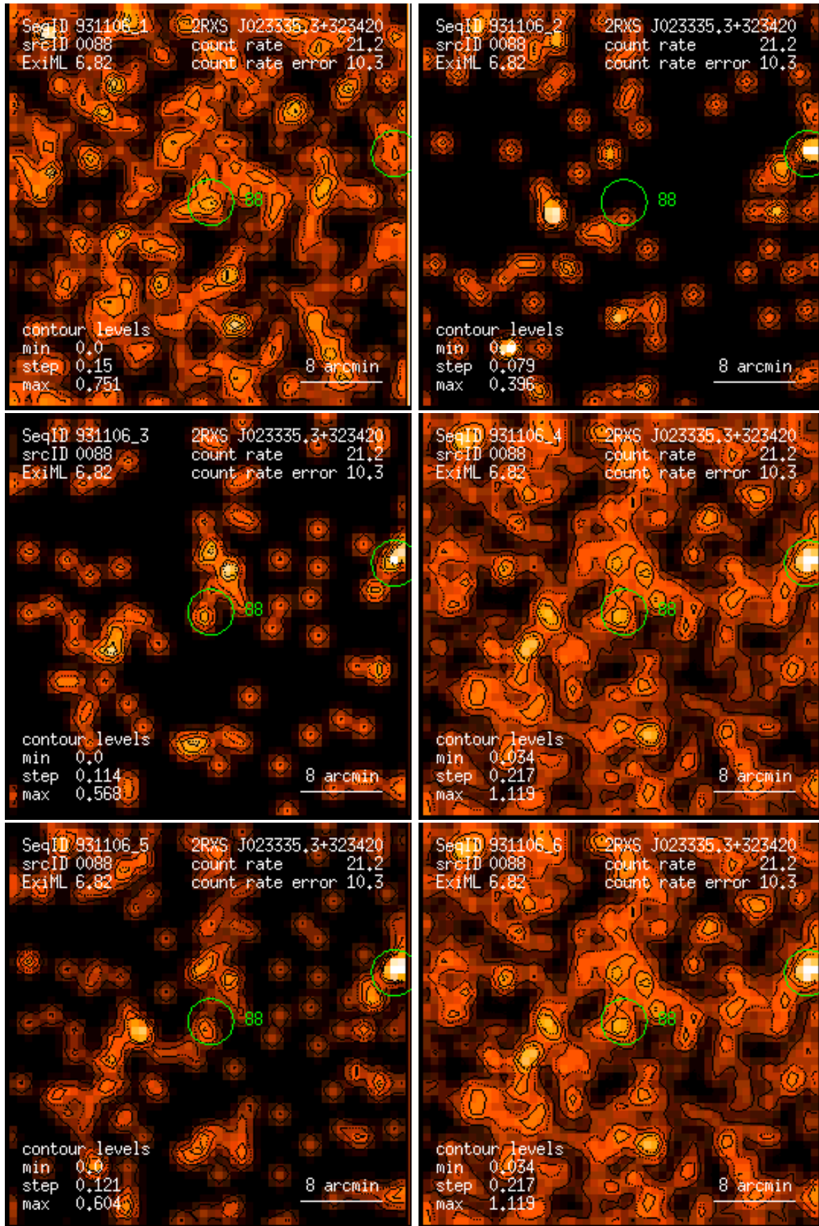
Figure 88: RASS 931106: detection 0088: band rate images, Gaussian filter: (1) PSPC channels 11 – 41, (2) 52 – 90, (3) 91 – 201, (4) 11 – 235, (5) 52 – 201, (6) 11 – 201. Broad band rates in counts/ks. Band rate contour levels in counts/ks/arcmin 2 .
