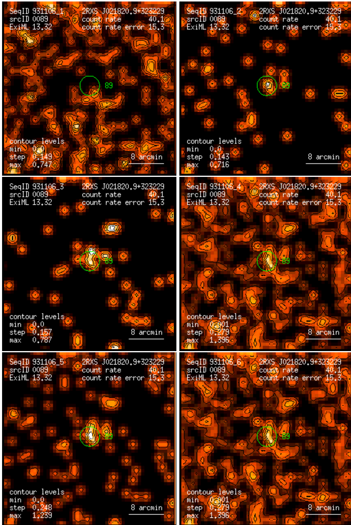
Figure 89: RASS 931106: detection 0089: band rate images, Gaussian filter: (1) PSPC channels 11 – 41, (2) 52 – 90, (3) 91 – 201, (4) 11 – 235, (5) 52 – 201, (6) 11 – 201. Broad band rates in counts/ks. Band rate contour levels in counts/ks/arcmin 2 .
