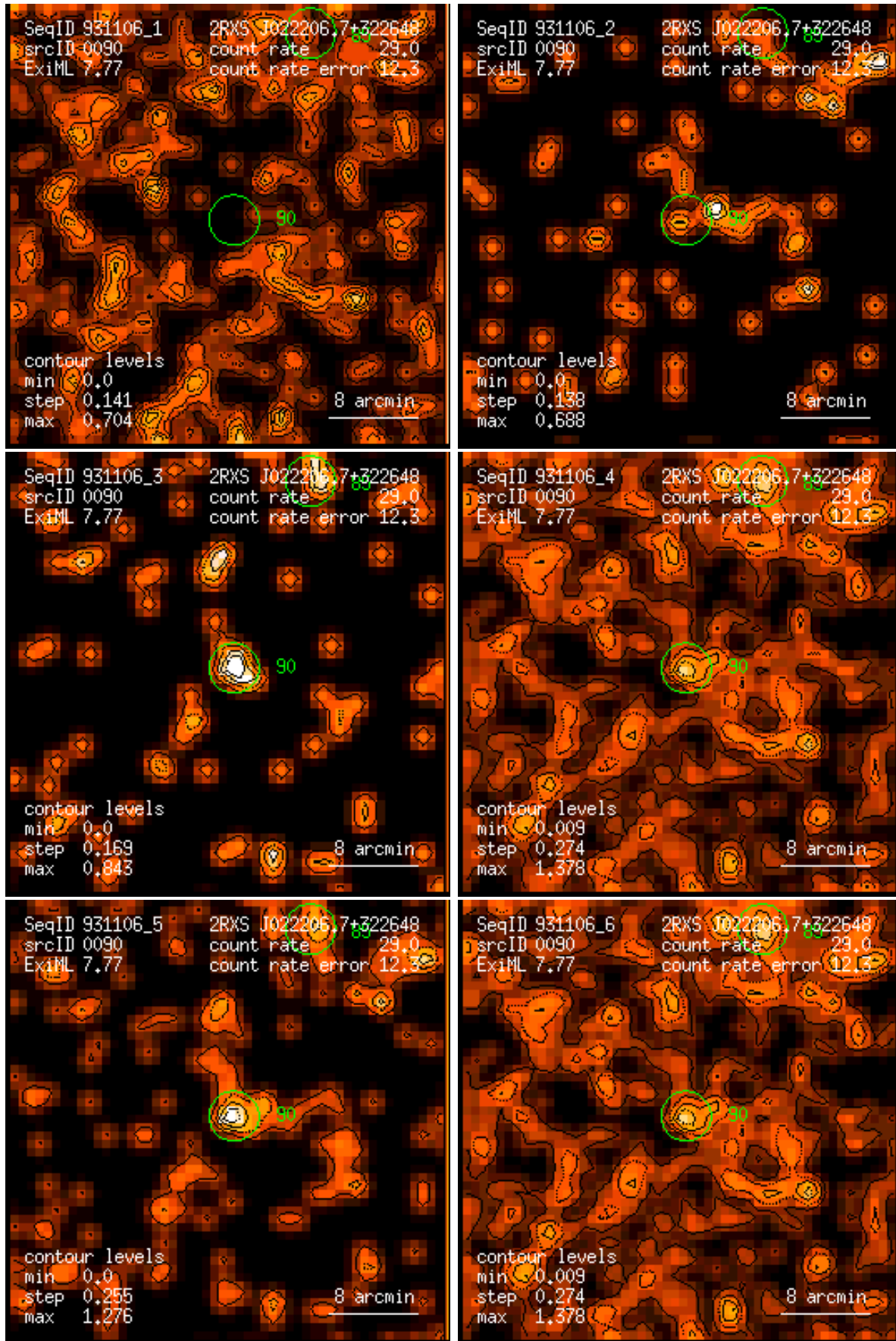
Figure 90: RASS 931106: detection 0090: band rate images, Gaussian filter: (1) PSPC channels 11 – 41, (2) 52 – 90, (3) 91 – 201, (4) 11 – 235, (5) 52 – 201, (6) 11 – 201. Broad band rates in counts/ks. Band rate contour levels in counts/ks/arcmin 2 .
