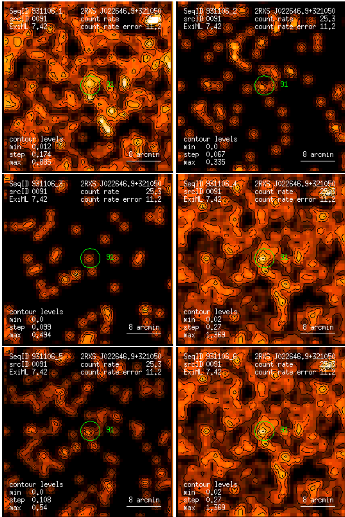
Figure 91: RASS 931106: detection 0091: band rate images, Gaussian filter: (1) PSPC channels 11 – 41, (2) 52 – 90, (3) 91 – 201, (4) 11 – 235, (5) 52 – 201, (6) 11 – 201. Broad band rates in counts/ks. Band rate contour levels in counts/ks/arcmin 2 .
