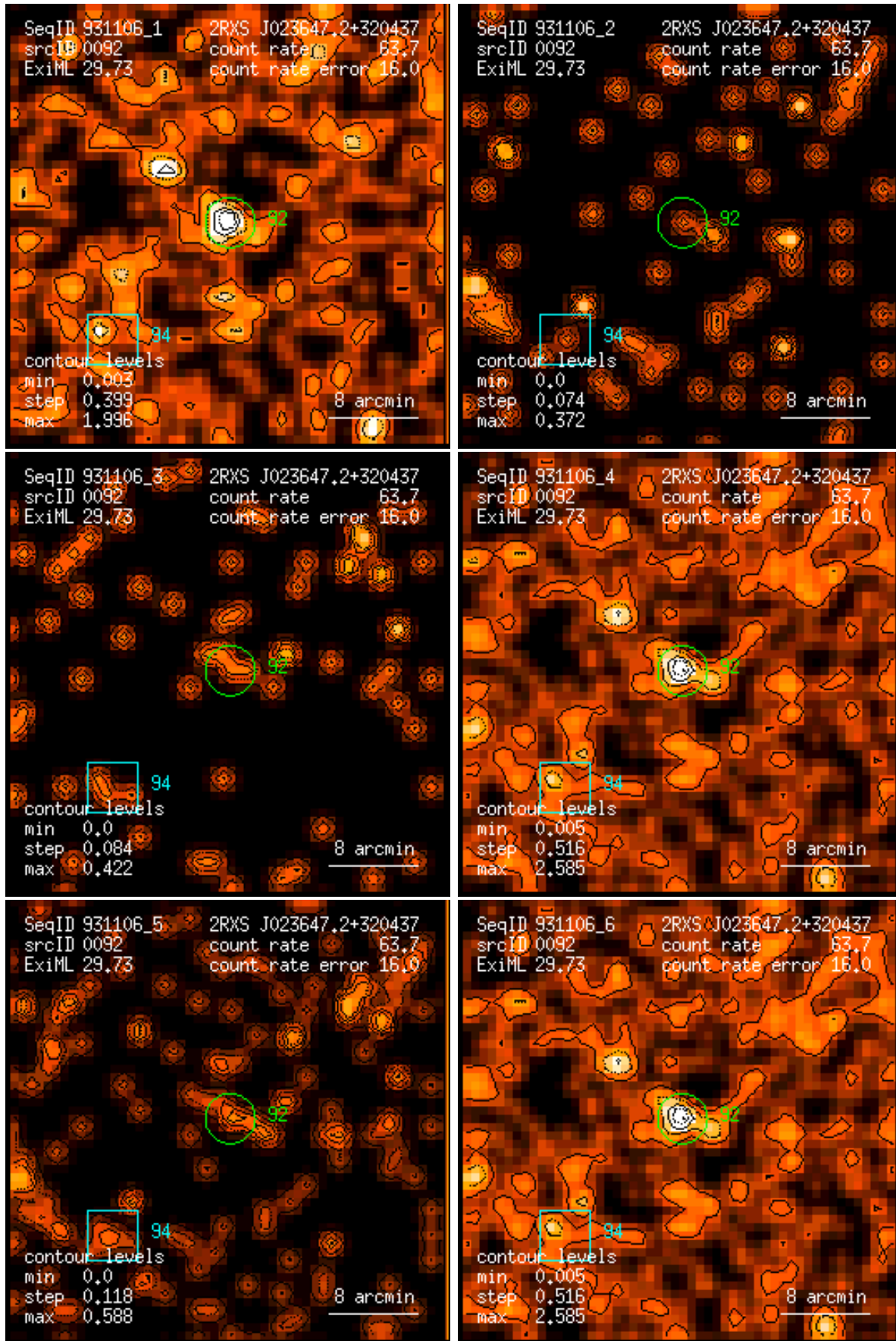
Figure 92: RASS 931106: detection 0092: band rate images, Gaussian filter: (1) PSPC channels 11 – 41, (2) 52 – 90, (3) 91 – 201, (4) 11 – 235, (5) 52 – 201, (6) 11 – 201. Broad band rates in counts/ks. Band rate contour levels in counts/ks/arcmin 2 .
