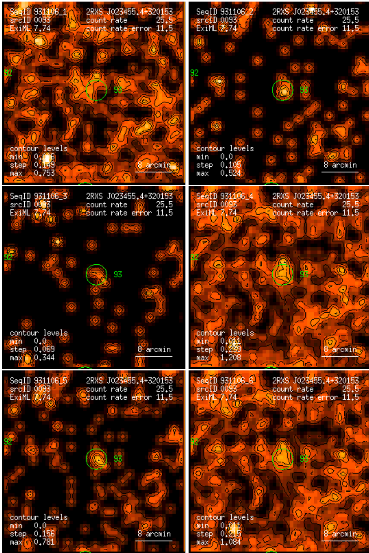
Figure 93: RASS 931106: detection 0093: band rate images, Gaussian filter: (1) PSPC channels 11 – 41, (2) 52 – 90, (3) 91 – 201, (4) 11 – 235, (5) 52 – 201, (6) 11 – 201. Broad band rates in counts/ks. Band rate contour levels in counts/ks/arcmin 2 .
