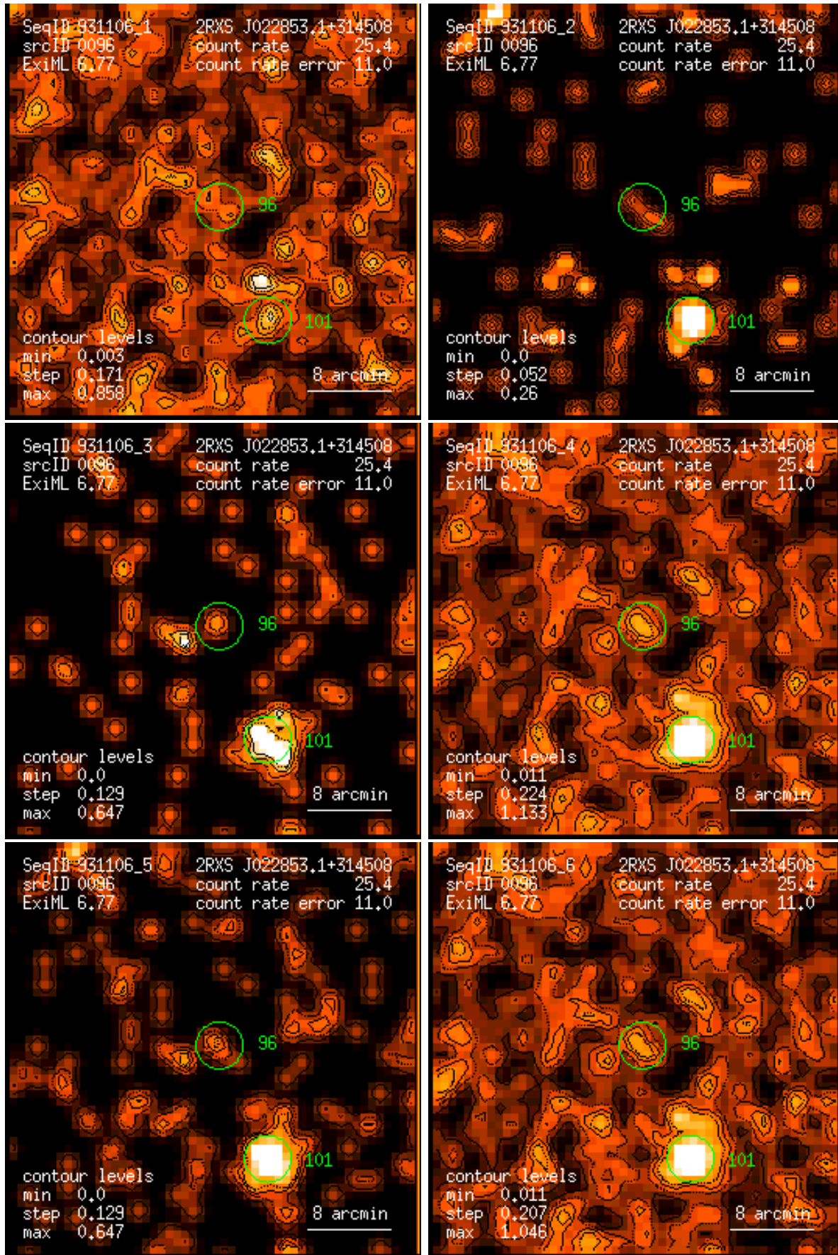
Figure 96: RASS 931106: detection 0096: band rate images, Gaussian filter: (1) PSPC channels 11 – 41, (2) 52 – 90, (3) 91 – 201, (4) 11 – 235, (5) 52 – 201, (6) 11 – 201. Broad band rates in counts/ks. Band rate contour levels in counts/ks/arcmin 2 .
