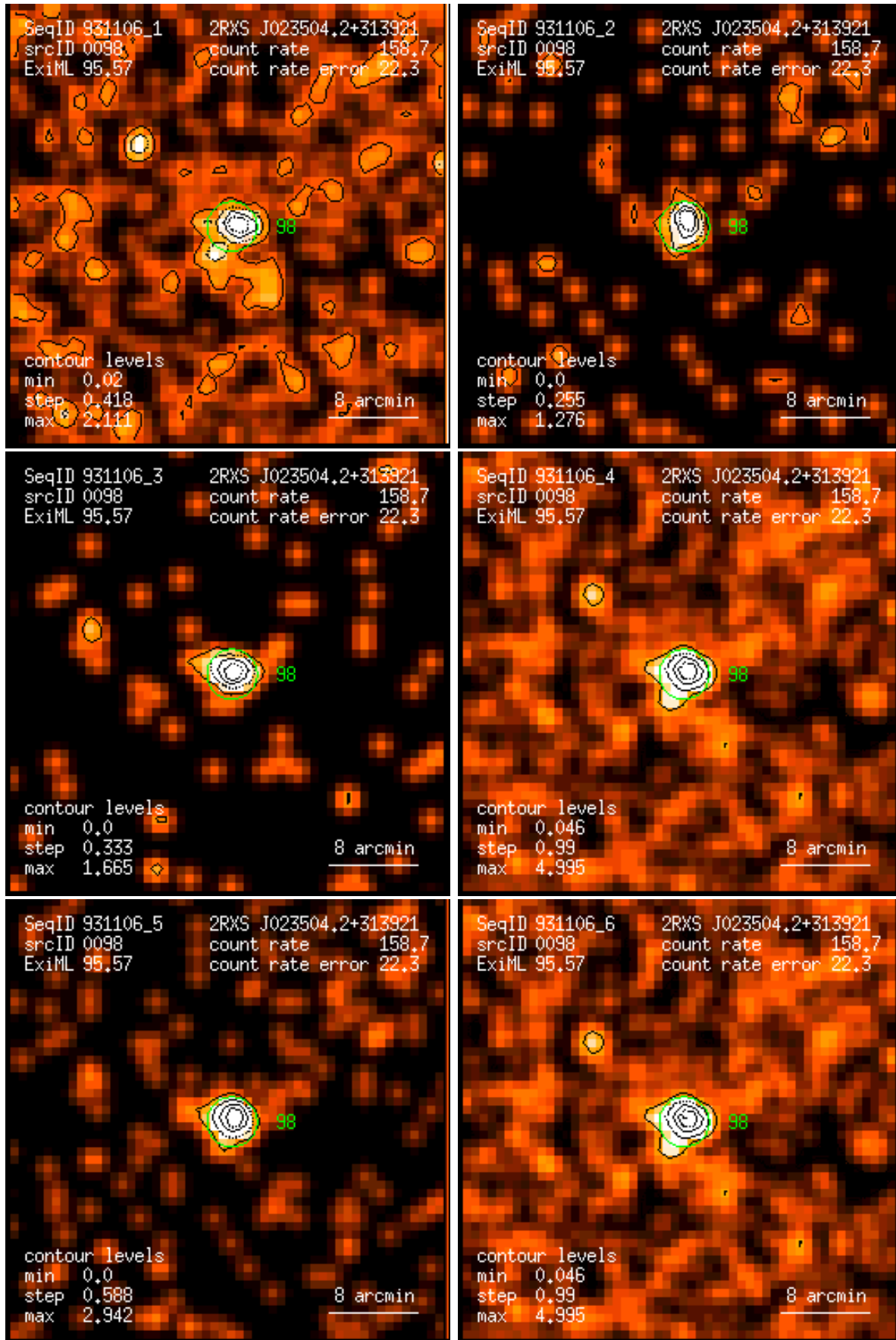
Figure 98: RASS 931106: detection 0098: band rate images, Gaussian filter: (1) PSPC channels 11 – 41, (2) 52 – 90, (3) 91 – 201, (4) 11 – 235, (5) 52 – 201, (6) 11 – 201. Broad band rates in counts/ks. Band rate contour levels in counts/ks/arcmin 2 .
