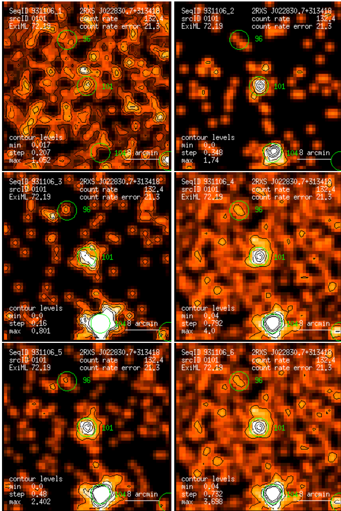
Figure 101: RASS 931106: detection 0101: band rate images, Gaussian filter: (1) PSPC channels 11 – 41, (2) 52 – 90, (3) 91 – 201, (4) 11 – 235, (5) 52 – 201, (6) 11 – 201. Broad band rates in counts/ks. Band rate contour levels in counts/ks/arcmin 2 .
