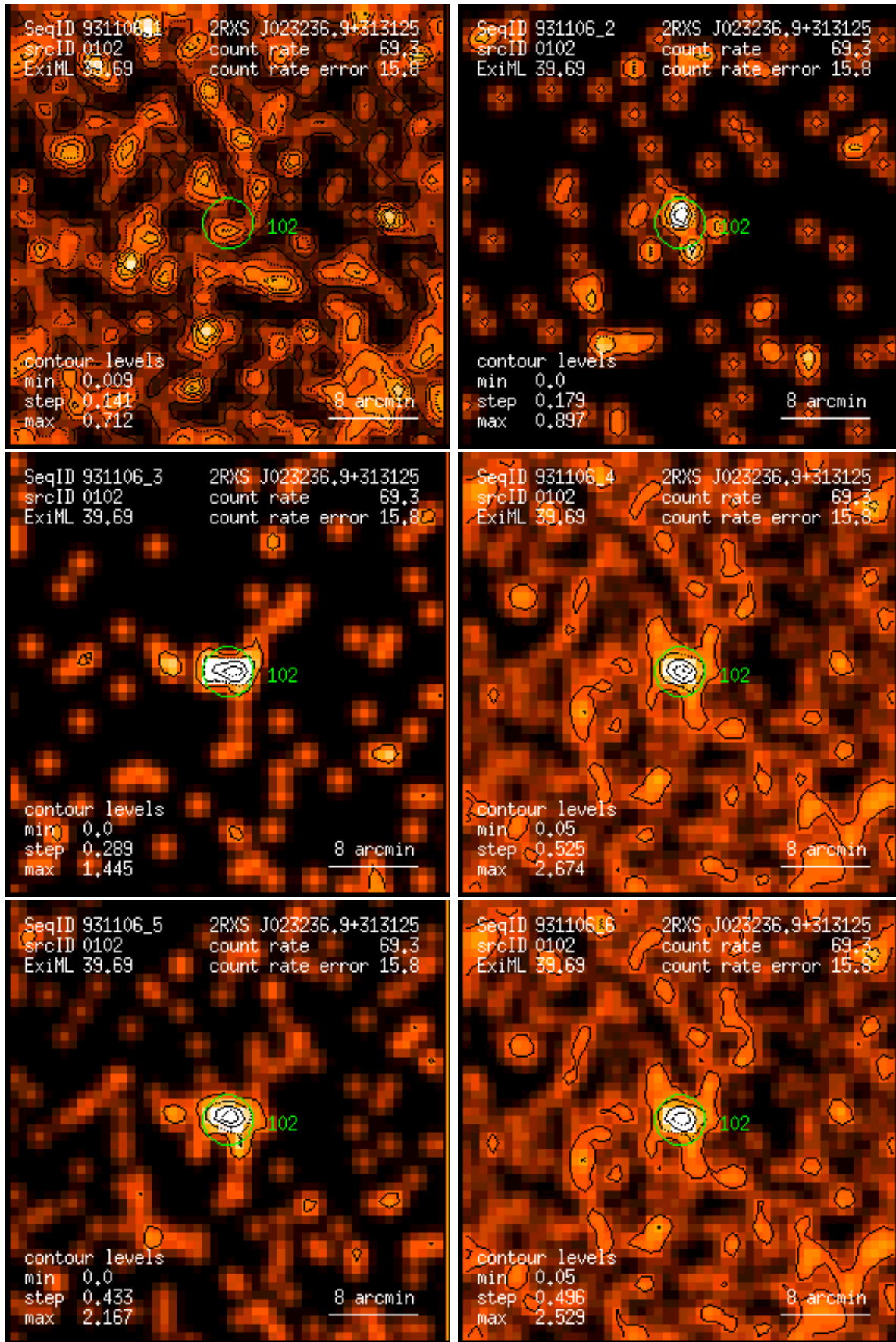
Figure 102: RASS 931106: detection 0102: band rate images, Gaussian filter: (1) PSPC channels 11 – 41, (2) 52 – 90, (3) 91 – 201, (4) 11 – 235, (5) 52 – 201, (6) 11 – 201. Broad band rates in counts/ks. Band rate contour levels in counts/ks/arcmin 2 .
