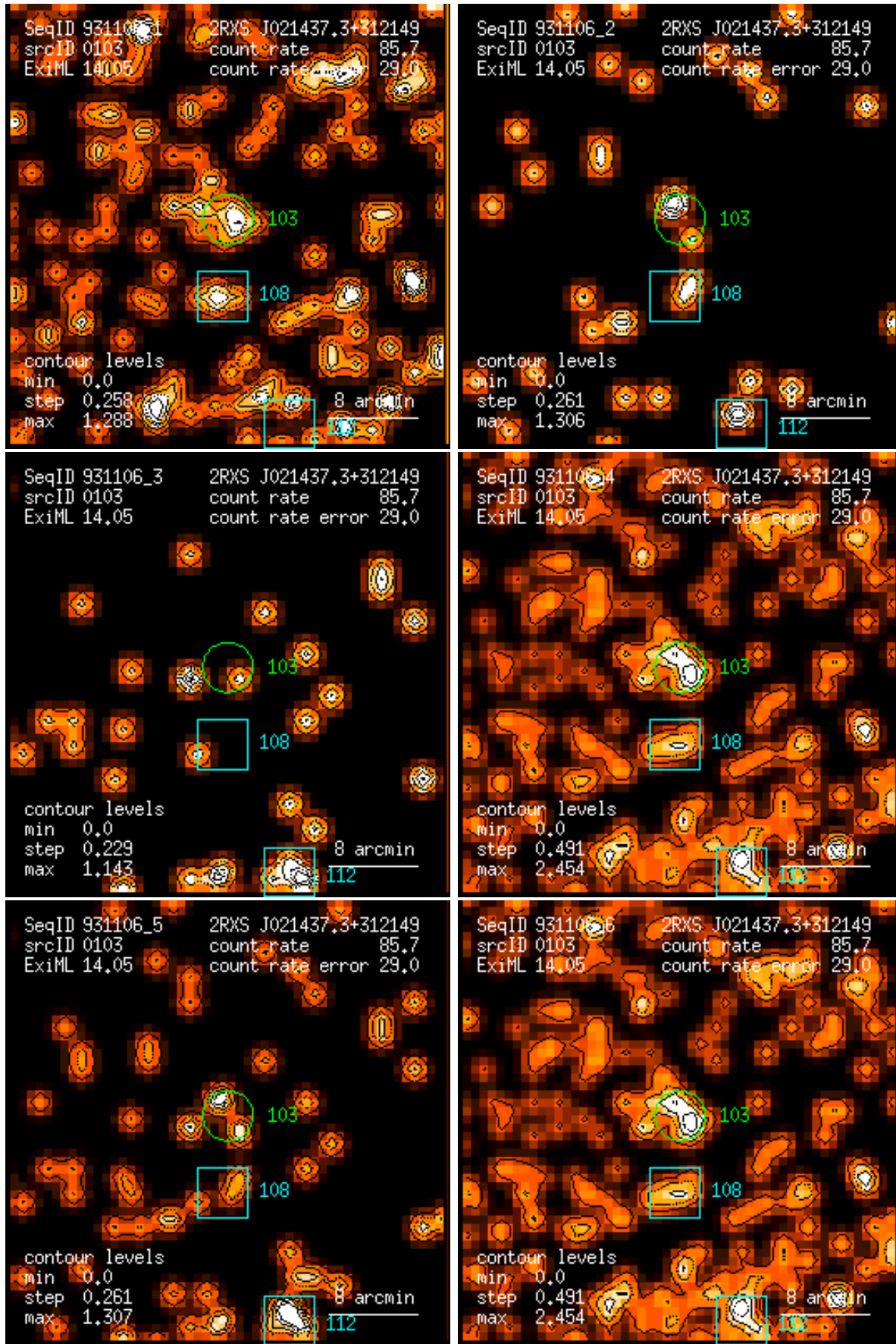
Figure 103: RASS 931106: detection 0103: band rate images, Gaussian filter: (1) PSPC channels 11 – 41, (2) 52 – 90, (3) 91 – 201, (4) 11 – 235, (5) 52 – 201, (6) 11 – 201. Broad band rates in counts/ks. Band rate contour levels in counts/ks/arcmin 2 .
