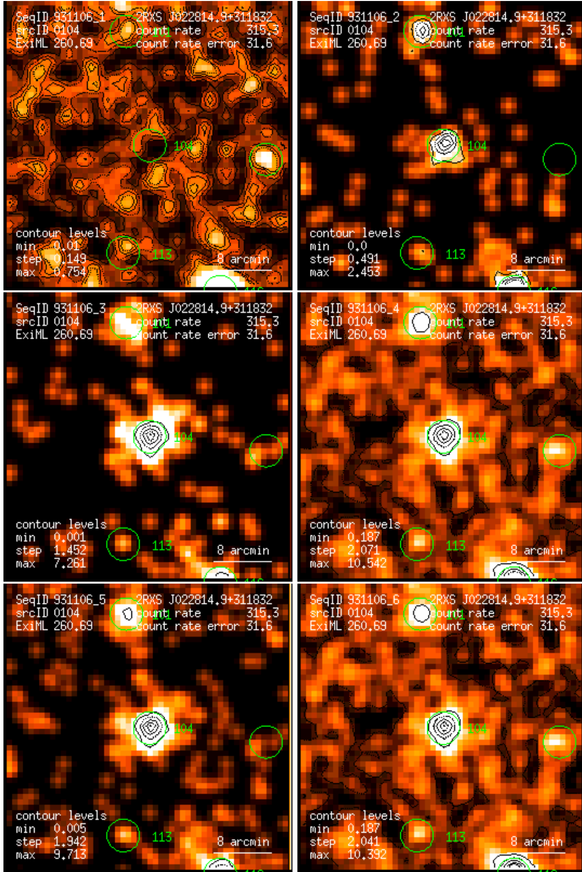
Figure 104: RASS 931106: detection 0104: band rate images, Gaussian filter: (1) PSPC channels 11 – 41, (2) 52 – 90, (3) 91 – 201, (4) 11 – 235, (5) 52 – 201, (6) 11 – 201. Broad band rates in counts/ks. Band rate contour levels in counts/ks/arcmin 2 .
