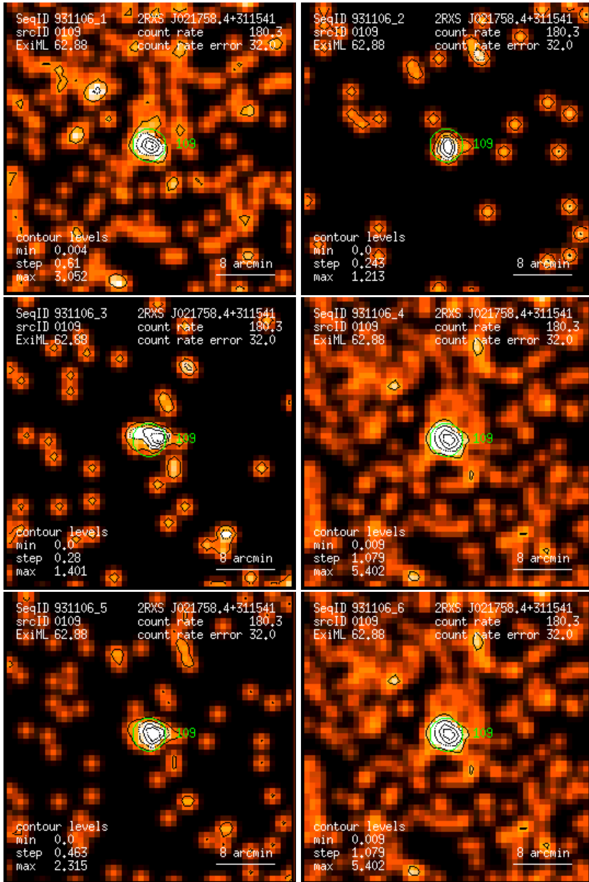
Figure 109: RASS 931106: detection 0109: band rate images, Gaussian filter: (1) PSPC channels 11 – 41, (2) 52 – 90, (3) 91 – 201, (4) 11 – 235, (5) 52 – 201, (6) 11 – 201. Broad band rates in counts/ks. Band rate contour levels in counts/ks/arcmin 2 .
