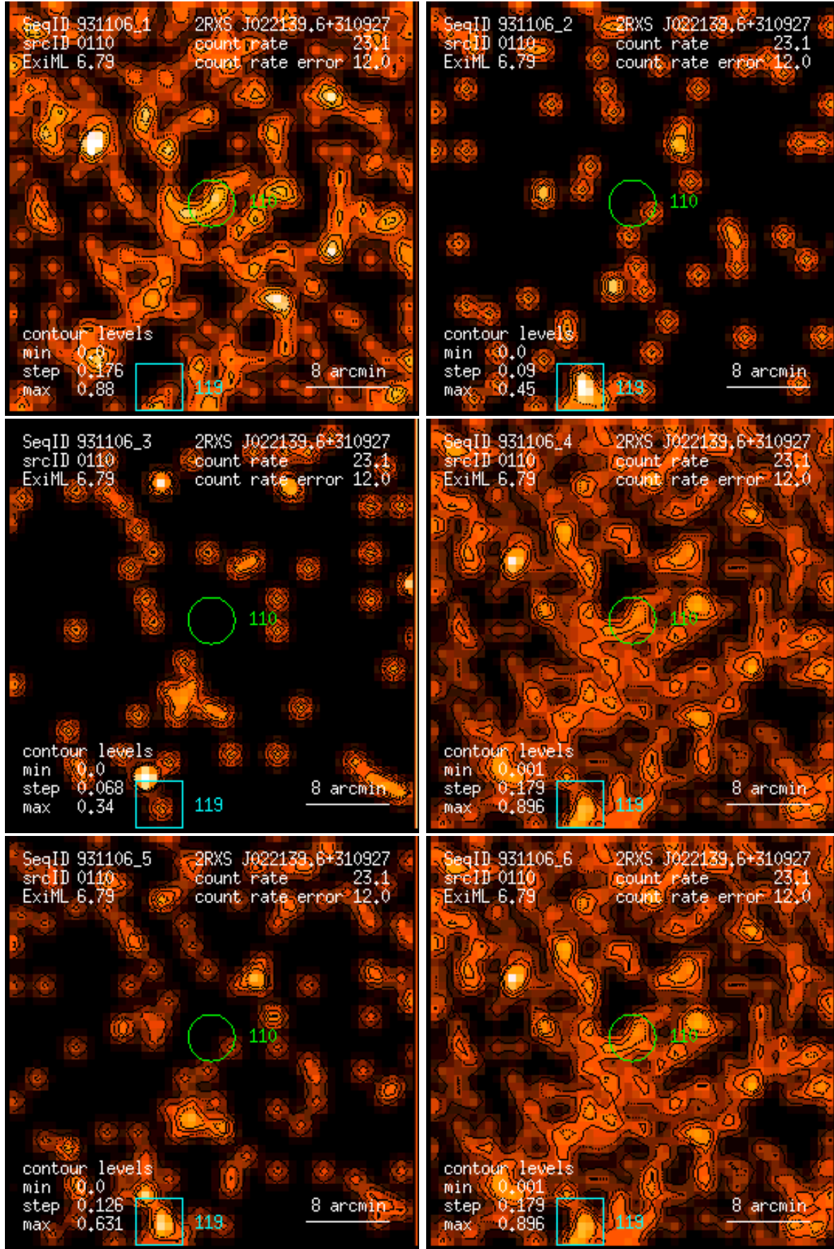
Figure 110: RASS 931106: detection 0110: band rate images, Gaussian filter: (1) PSPC channels 11 – 41, (2) 52 – 90, (3) 91 – 201, (4) 11 – 235, (5) 52 – 201, (6) 11 – 201. Broad band rates in counts/ks. Band rate contour levels in counts/ks/arcmin 2 .
