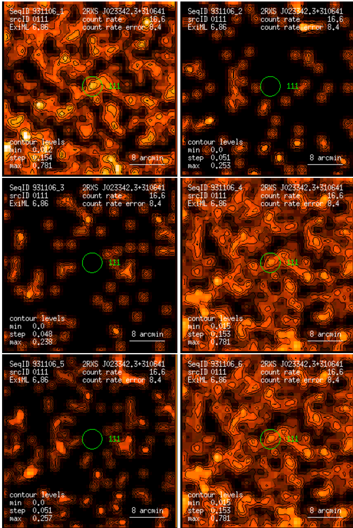
Figure 111: RASS 931106: detection 0111: band rate images, Gaussian filter: (1) PSPC channels 11 – 41, (2) 52 – 90, (3) 91 – 201, (4) 11 – 235, (5) 52 – 201, (6) 11 – 201. Broad band rates in counts/ks. Band rate contour levels in counts/ks/arcmin 2 .
