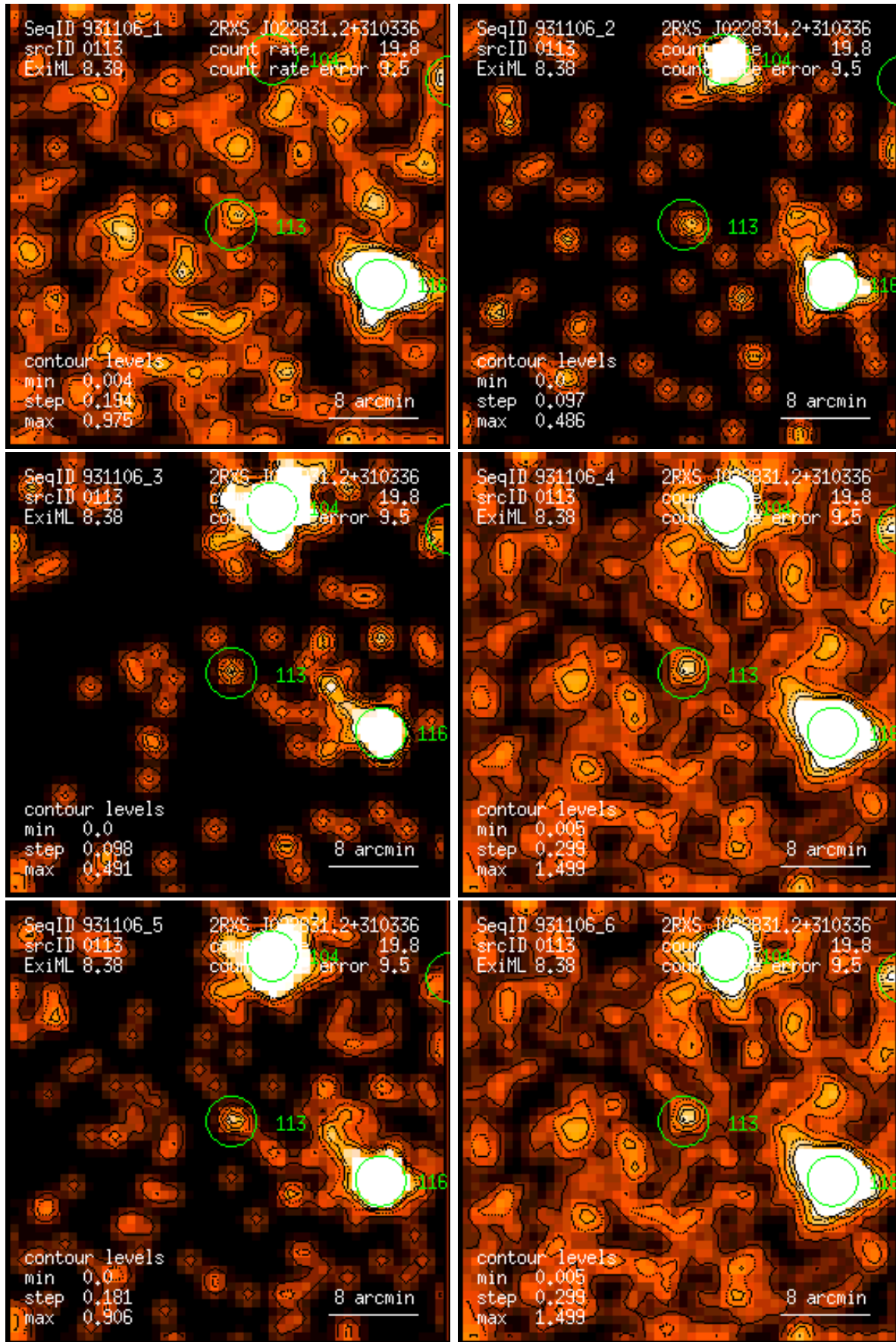
Figure 113: RASS 931106: detection 0113: band rate images, Gaussian filter: (1) PSPC channels 11 – 41, (2) 52 – 90, (3) 91 – 201, (4) 11 – 235, (5) 52 – 201, (6) 11 – 201. Broad band rates in counts/ks. Band rate contour levels in counts/ks/arcmin 2 .
