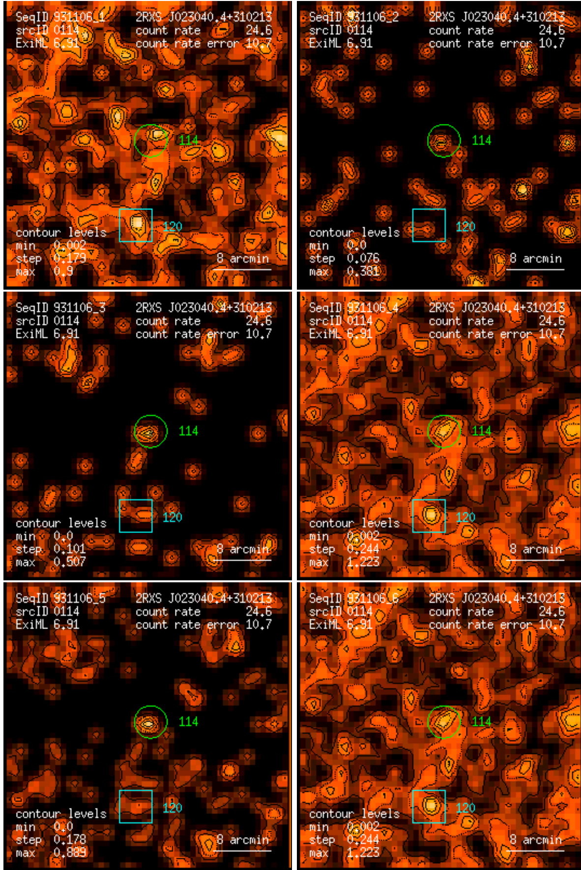
Figure 114: RASS 931106: detection 0114: band rate images, Gaussian filter: (1) PSPC channels 11 – 41, (2) 52 – 90, (3) 91 – 201, (4) 11 – 235, (5) 52 – 201, (6) 11 – 201. Broad band rates in counts/ks. Band rate contour levels in counts/ks/arcmin 2 .
