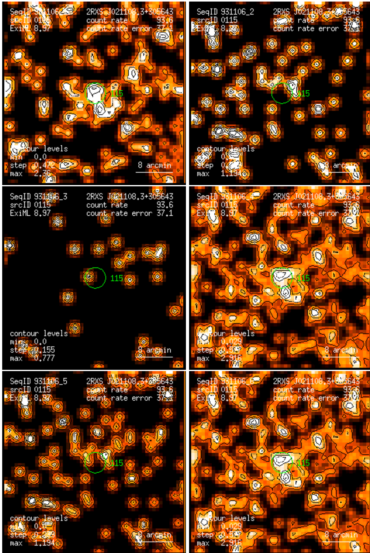
Figure 115: RASS 931106: detection 0115: band rate images, Gaussian filter: (1) PSPC channels 11 – 41, (2) 52 – 90, (3) 91 – 201, (4) 11 – 235, (5) 52 – 201, (6) 11 – 201. Broad band rates in counts/ks. Band rate contour levels in counts/ks/arcmin 2 .
