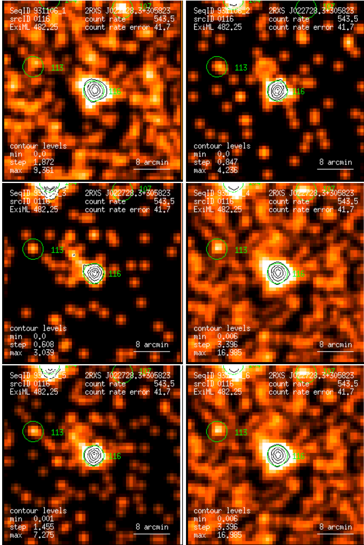
Figure 116: RASS 931106: detection 0116: band rate images, Gaussian filter: (1) PSPC channels 11 – 41, (2) 52 – 90, (3) 91 – 201, (4) 11 – 235, (5) 52 – 201, (6) 11 – 201. Broad band rates in counts/ks. Band rate contour levels in counts/ks/arcmin 2 .
