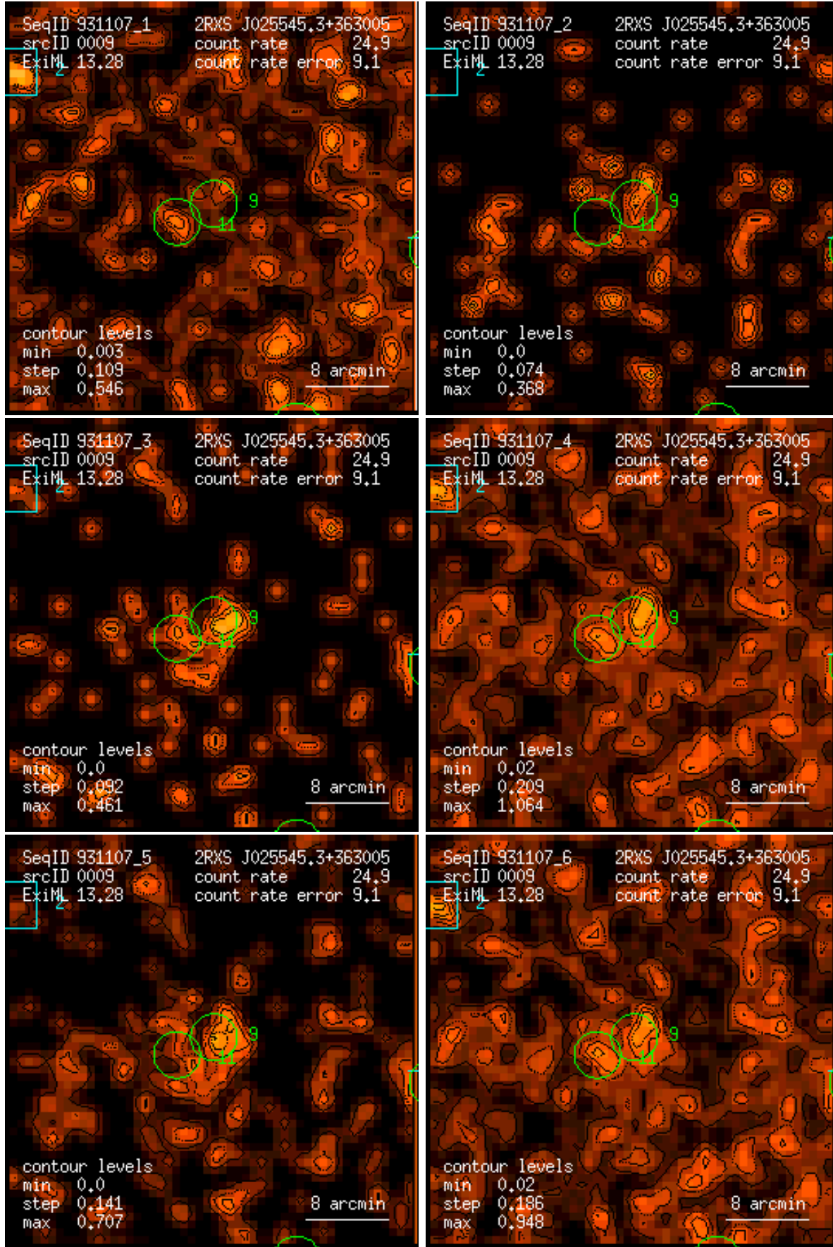
Figure 9: RASS 931107: detection 0009: band rate images, Gaussian filter: (1) PSPC channels 11 – 41, (2) 52 – 90, (3) 91 – 201, (4) 11 – 235, (5) 52 – 201, (6) 11 – 201. Broad band rates in counts/ks. Band rate contour levels in counts/ks/arcmin 2 .
