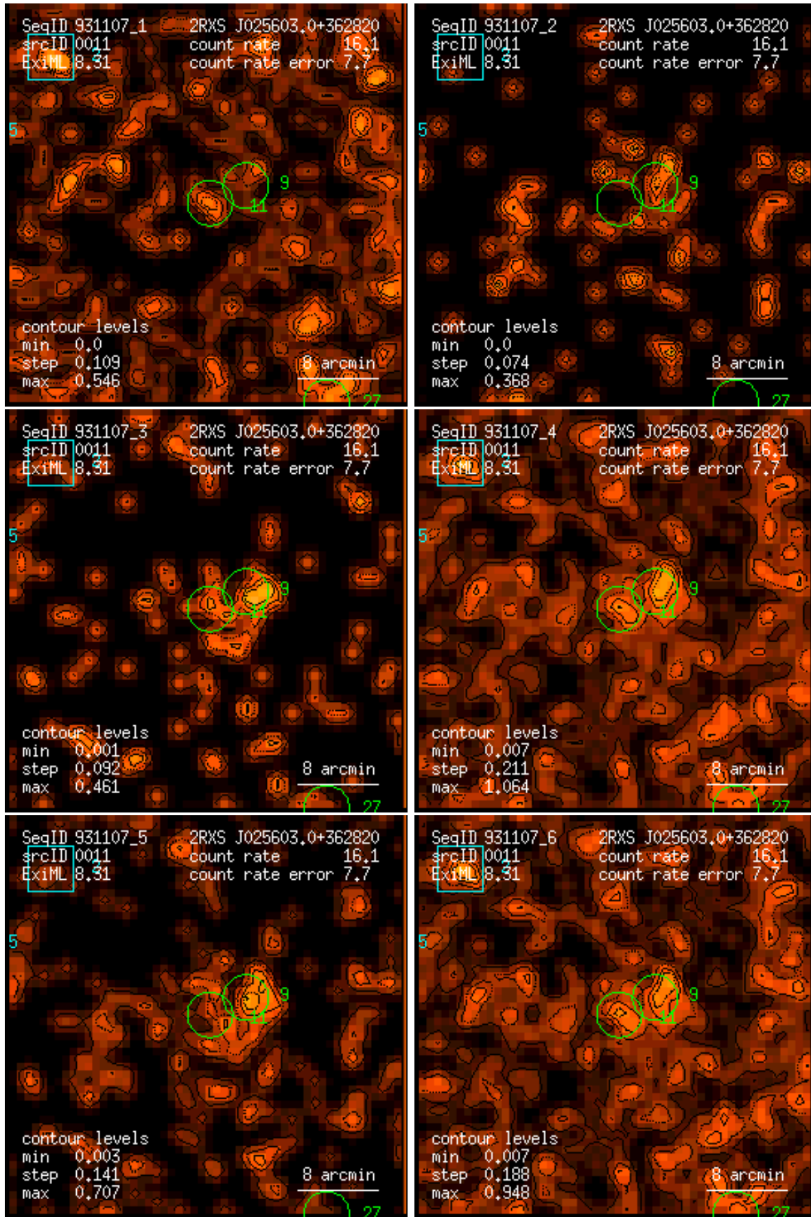
Figure 11: RASS 931107: detection 0011: band rate images, Gaussian filter: (1) PSPC channels 11 – 41, (2) 52 – 90, (3) 91 – 201, (4) 11 – 235, (5) 52 – 201, (6) 11 – 201. Broad band rates in counts/ks. Band rate contour levels in counts/ks/arcmin 2 .
