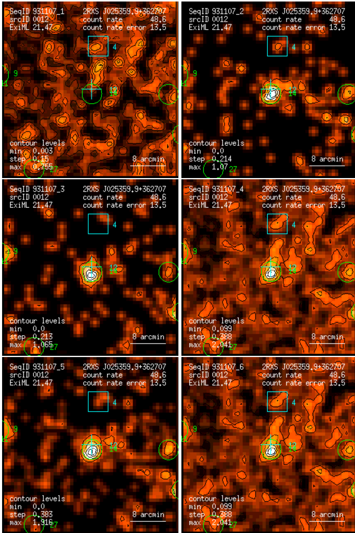
Figure 12: RASS 931107: detection 0012: band rate images, Gaussian filter: (1) PSPC channels 11 – 41, (2) 52 – 90, (3) 91 – 201, (4) 11 – 235, (5) 52 – 201, (6) 11 – 201. Broad band rates in counts/ks. Band rate contour levels in counts/ks/arcmin 2 .
