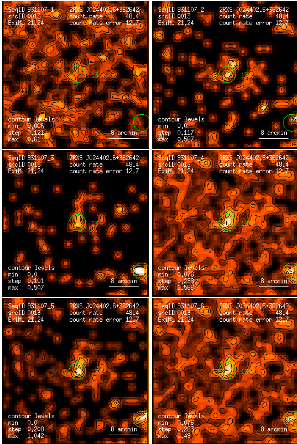
Figure 13: RASS 931107: detection 0013: band rate images, Gaussian filter: (1) PSPC channels 11 – 41, (2) 52 – 90, (3) 91 – 201, (4) 11 – 235, (5) 52 – 201, (6) 11 – 201. Broad band rates in counts/ks. Band rate contour levels in counts/ks/arcmin 2 .
