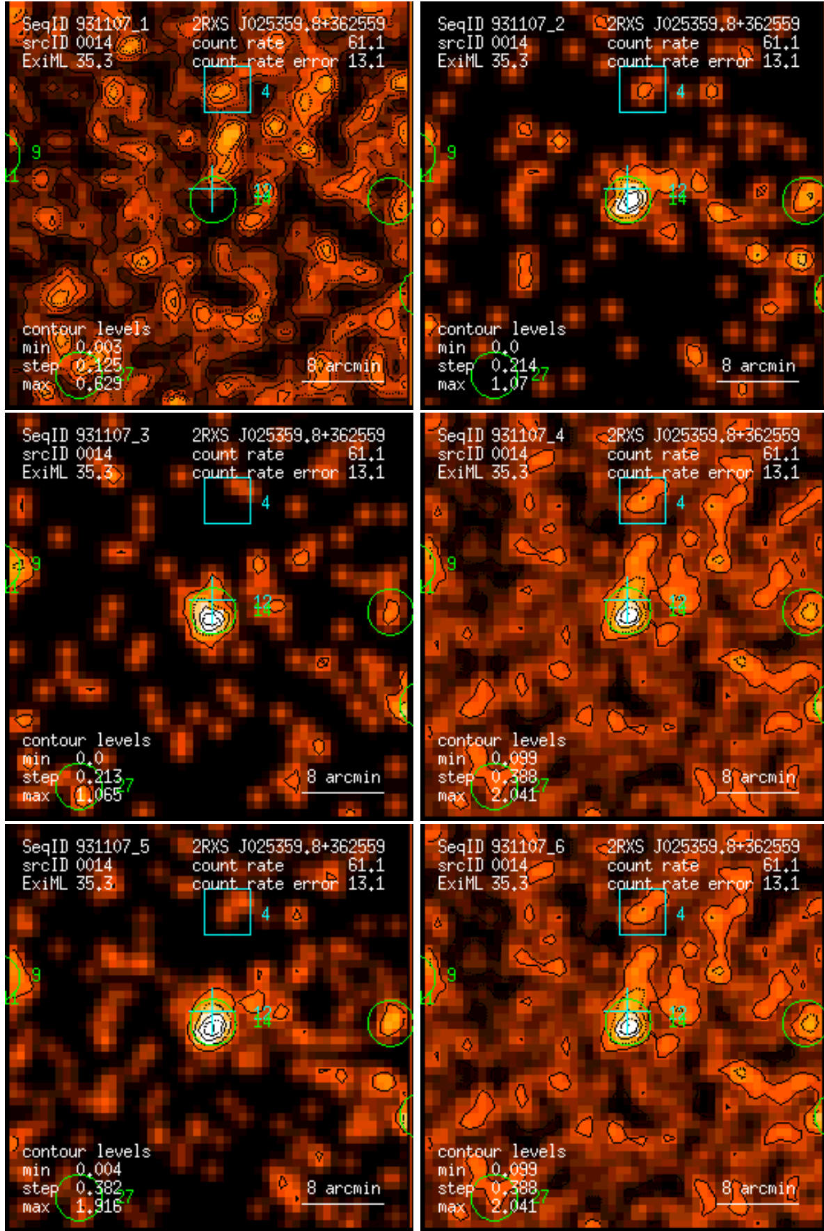
Figure 14: RASS 931107: detection 0014: band rate images, Gaussian filter: (1) PSPC channels 11 – 41, (2) 52 – 90, (3) 91 – 201, (4) 11 – 235, (5) 52 – 201, (6) 11 – 201. Broad band rates in counts/ks. Band rate contour levels in counts/ks/arcmin 2 .
