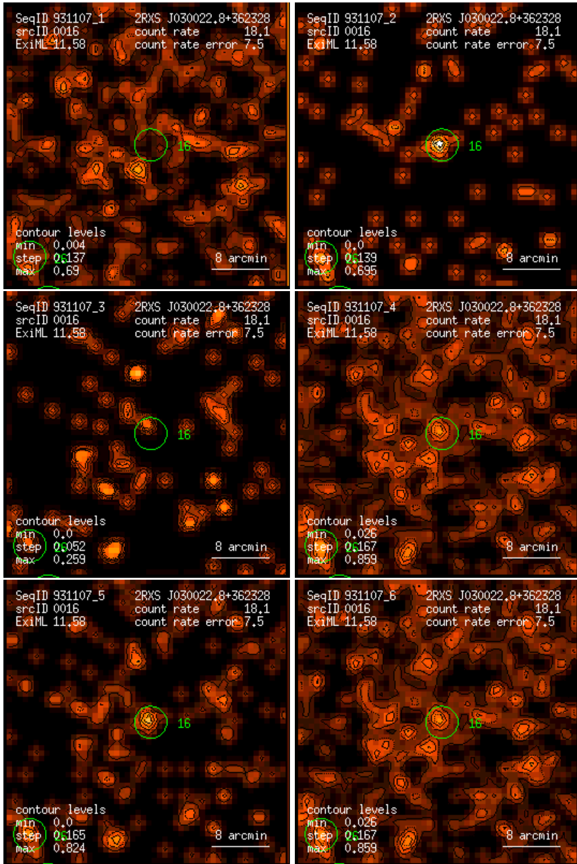
Figure 16: RASS 931107: detection 0016: band rate images, Gaussian filter: (1) PSPC channels 11 – 41, (2) 52 – 90, (3) 91 – 201, (4) 11 – 235, (5) 52 – 201, (6) 11 – 201. Broad band rates in counts/ks. Band rate contour levels in counts/ks/arcmin 2 .
