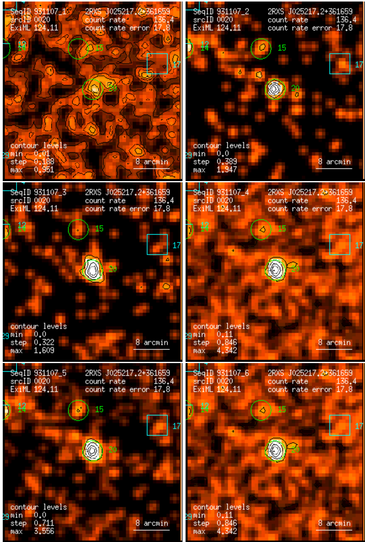
Figure 20: RASS 931107: detection 0020: band rate images, Gaussian filter: (1) PSPC channels 11 – 41, (2) 52 – 90, (3) 91 – 201, (4) 11 – 235, (5) 52 – 201, (6) 11 – 201. Broad band rates in counts/ks. Band rate contour levels in counts/ks/arcmin 2 .
