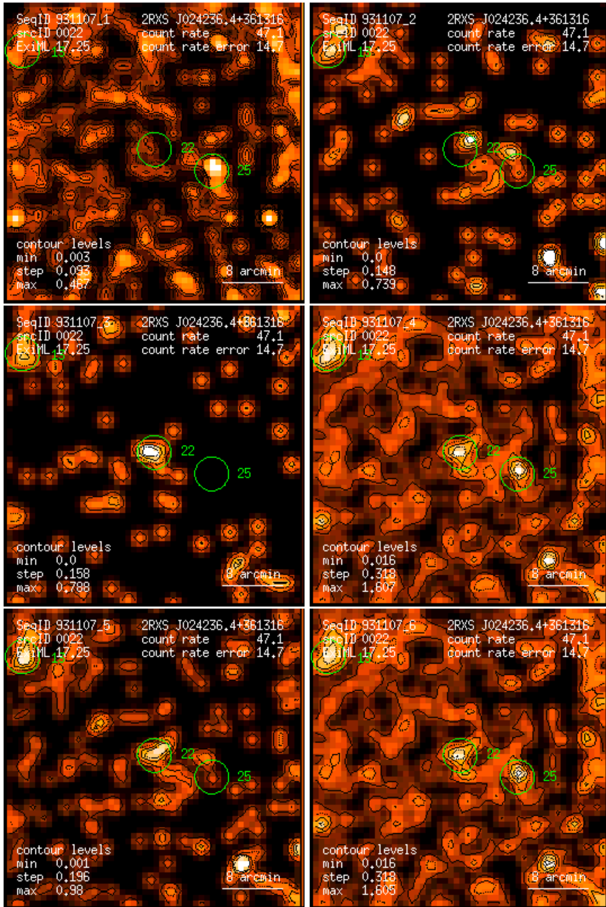
Figure 22: RASS 931107: detection 0022: band rate images, Gaussian filter: (1) PSPC channels 11 – 41, (2) 52 – 90, (3) 91 – 201, (4) 11 – 235, (5) 52 – 201, (6) 11 – 201. Broad band rates in counts/ks. Band rate contour levels in counts/ks/arcmin 2 .
