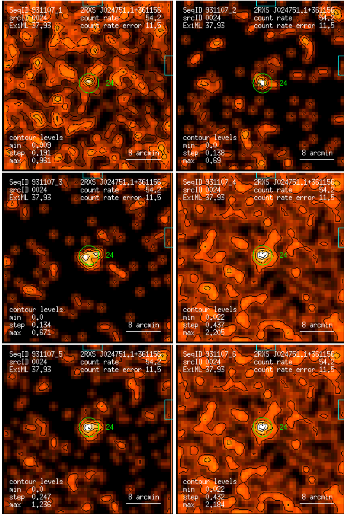
Figure 24: RASS 931107: detection 0024: band rate images, Gaussian filter: (1) PSPC channels 11 – 41, (2) 52 – 90, (3) 91 – 201, (4) 11 – 235, (5) 52 – 201, (6) 11 – 201. Broad band rates in counts/ks. Band rate contour levels in counts/ks/arcmin 2 .
