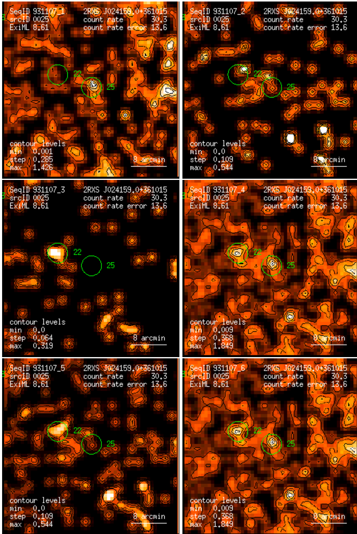
Figure 25: RASS 931107: detection 0025: band rate images, Gaussian filter: (1) PSPC channels 11 – 41, (2) 52 – 90, (3) 91 – 201, (4) 11 – 235, (5) 52 – 201, (6) 11 – 201. Broad band rates in counts/ks. Band rate contour levels in counts/ks/arcmin 2 .
