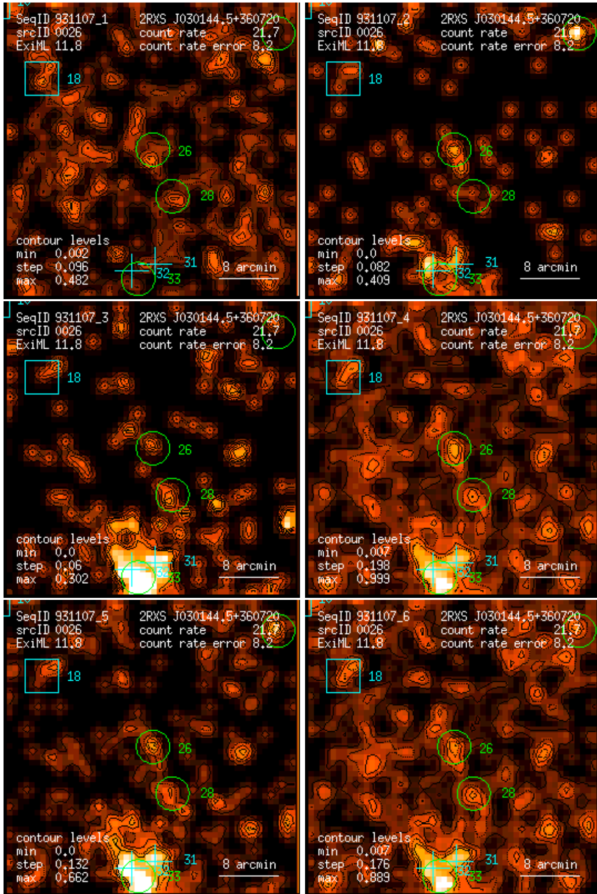
Figure 26: RASS 931107: detection 0026: band rate images, Gaussian filter: (1) PSPC channels 11 – 41, (2) 52 – 90, (3) 91 – 201, (4) 11 – 235, (5) 52 – 201, (6) 11 – 201. Broad band rates in counts/ks. Band rate contour levels in counts/ks/arcmin 2 .
