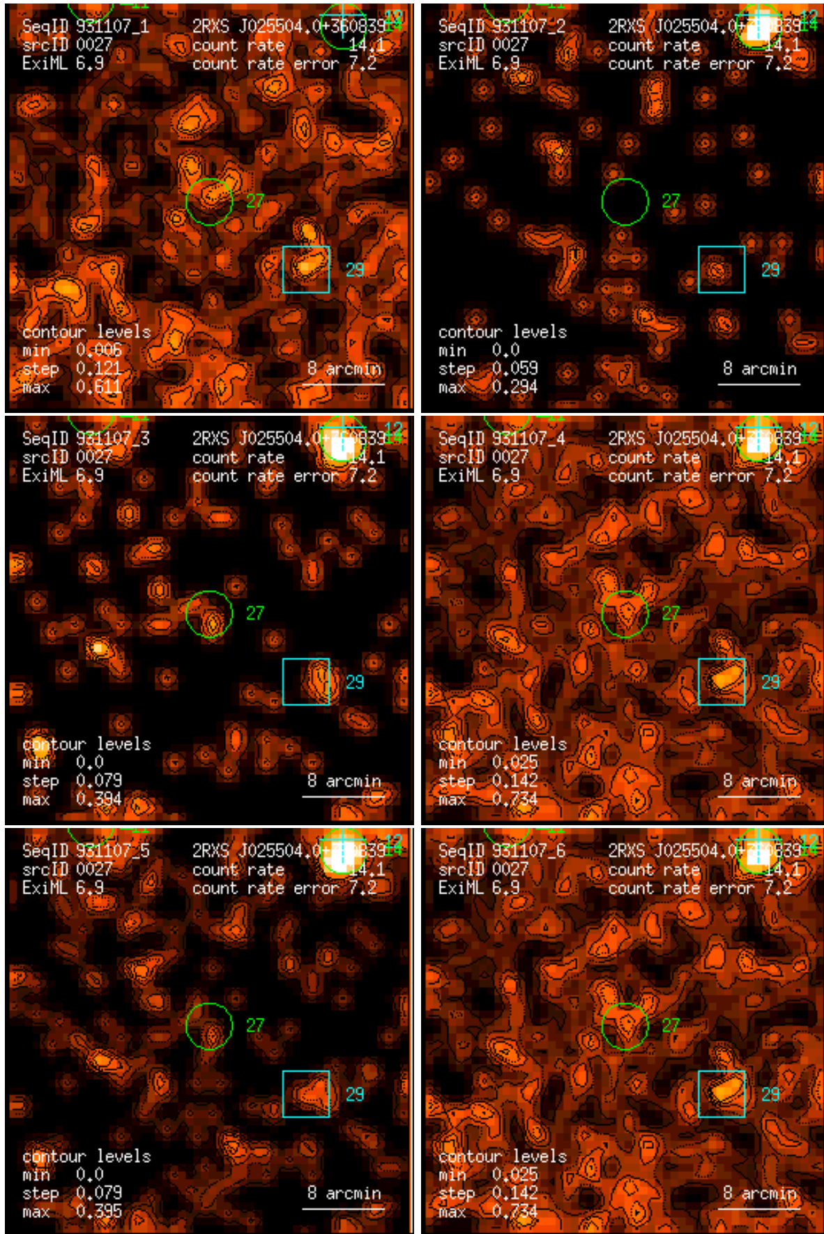
Figure 27: RASS 931107: detection 0027: band rate images, Gaussian filter: (1) PSPC channels 11 – 41, (2) 52 – 90, (3) 91 – 201, (4) 11 – 235, (5) 52 – 201, (6) 11 – 201. Broad band rates in counts/ks. Band rate contour levels in counts/ks/arcmin 2 .
