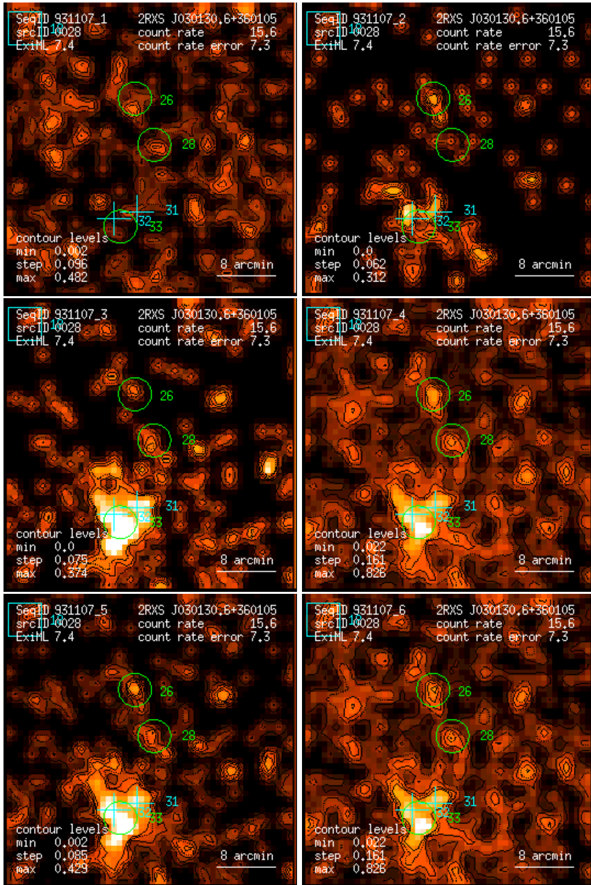
Figure 28: RASS 931107: detection 0028: band rate images, Gaussian filter: (1) PSPC channels 11 – 41, (2) 52 – 90, (3) 91 – 201, (4) 11 – 235, (5) 52 – 201, (6) 11 – 201. Broad band rates in counts/ks. Band rate contour levels in counts/ks/arcmin 2 .
