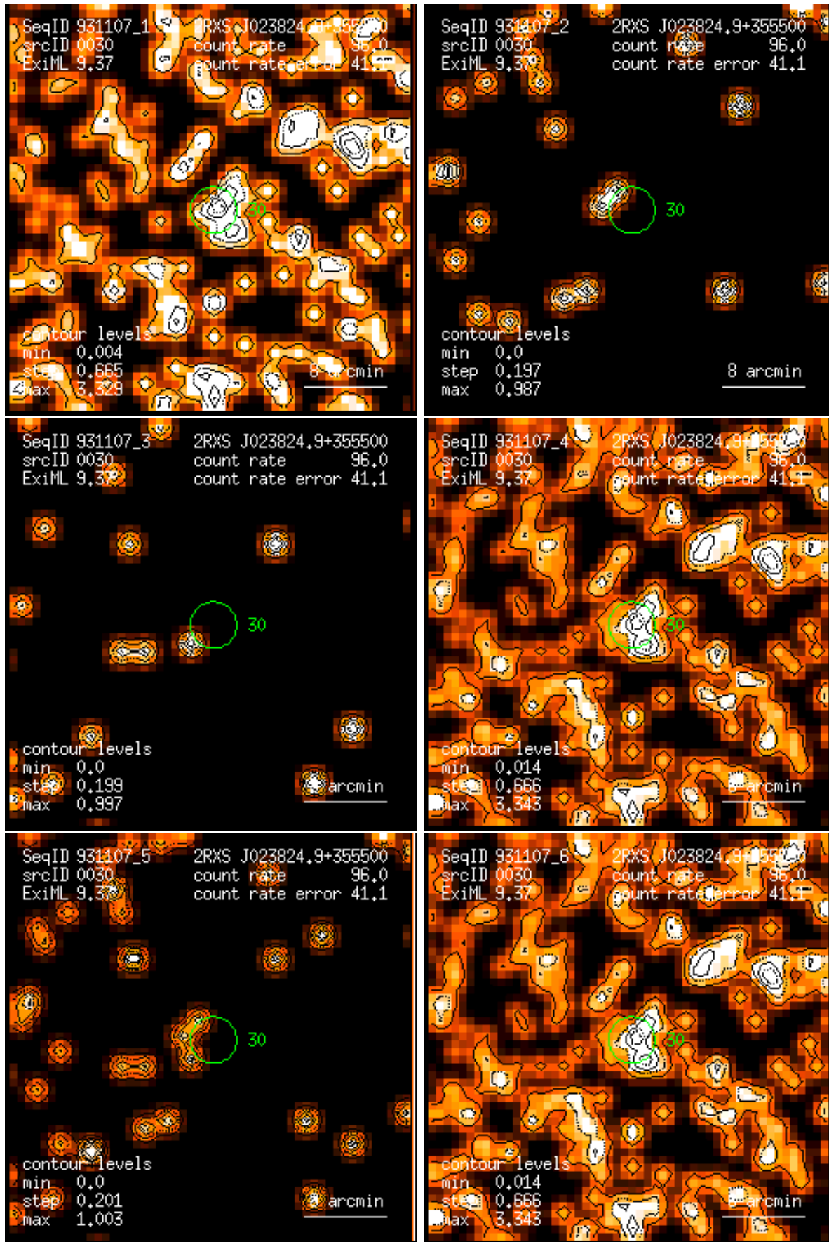
Figure 30: RASS 931107: detection 0030: band rate images, Gaussian filter: (1) PSPC channels 11 – 41, (2) 52 – 90, (3) 91 – 201, (4) 11 – 235, (5) 52 – 201, (6) 11 – 201. Broad band rates in counts/ks. Band rate contour levels in counts/ks/arcmin 2 .
