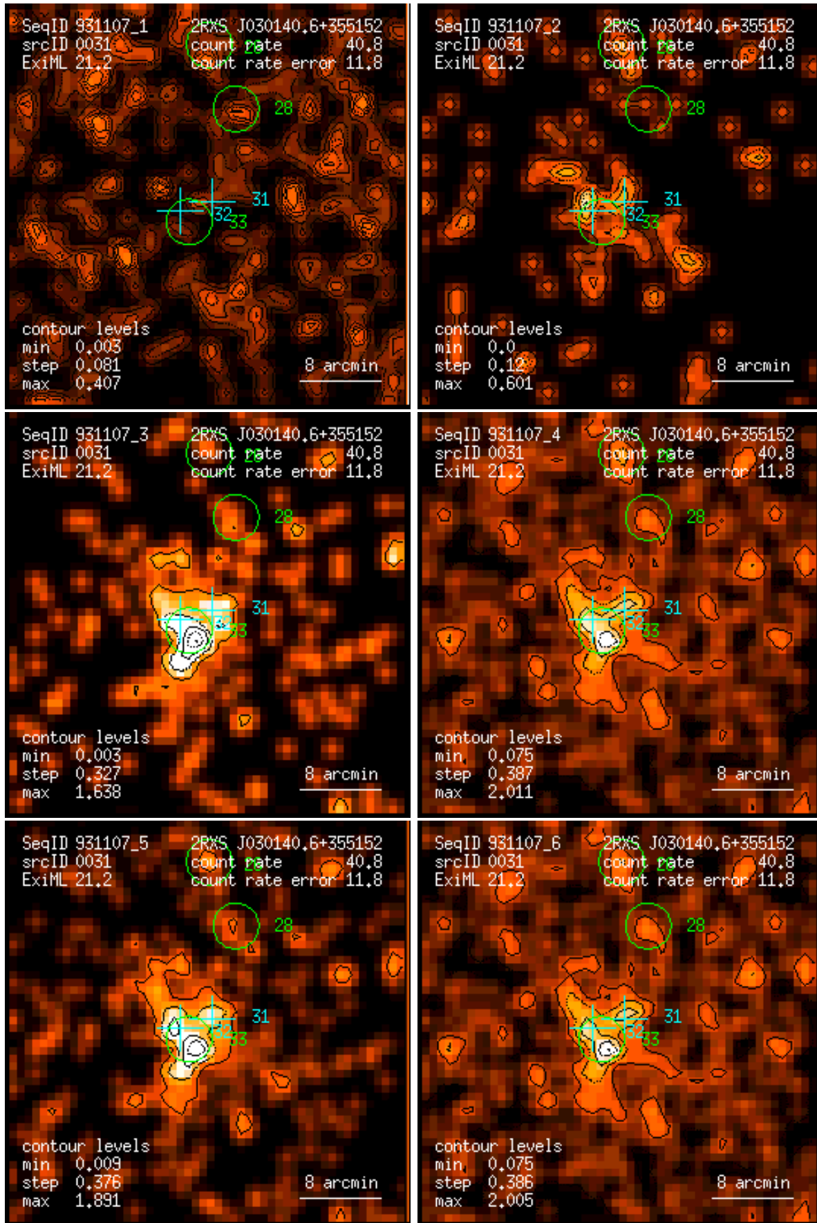
Figure 31: RASS 931107: detection 0031: band rate images, Gaussian filter: (1) PSPC channels 11 – 41, (2) 52 – 90, (3) 91 – 201, (4) 11 – 235, (5) 52 – 201, (6) 11 – 201. Broad band rates in counts/ks. Band rate contour levels in counts/ks/arcmin 2 .
