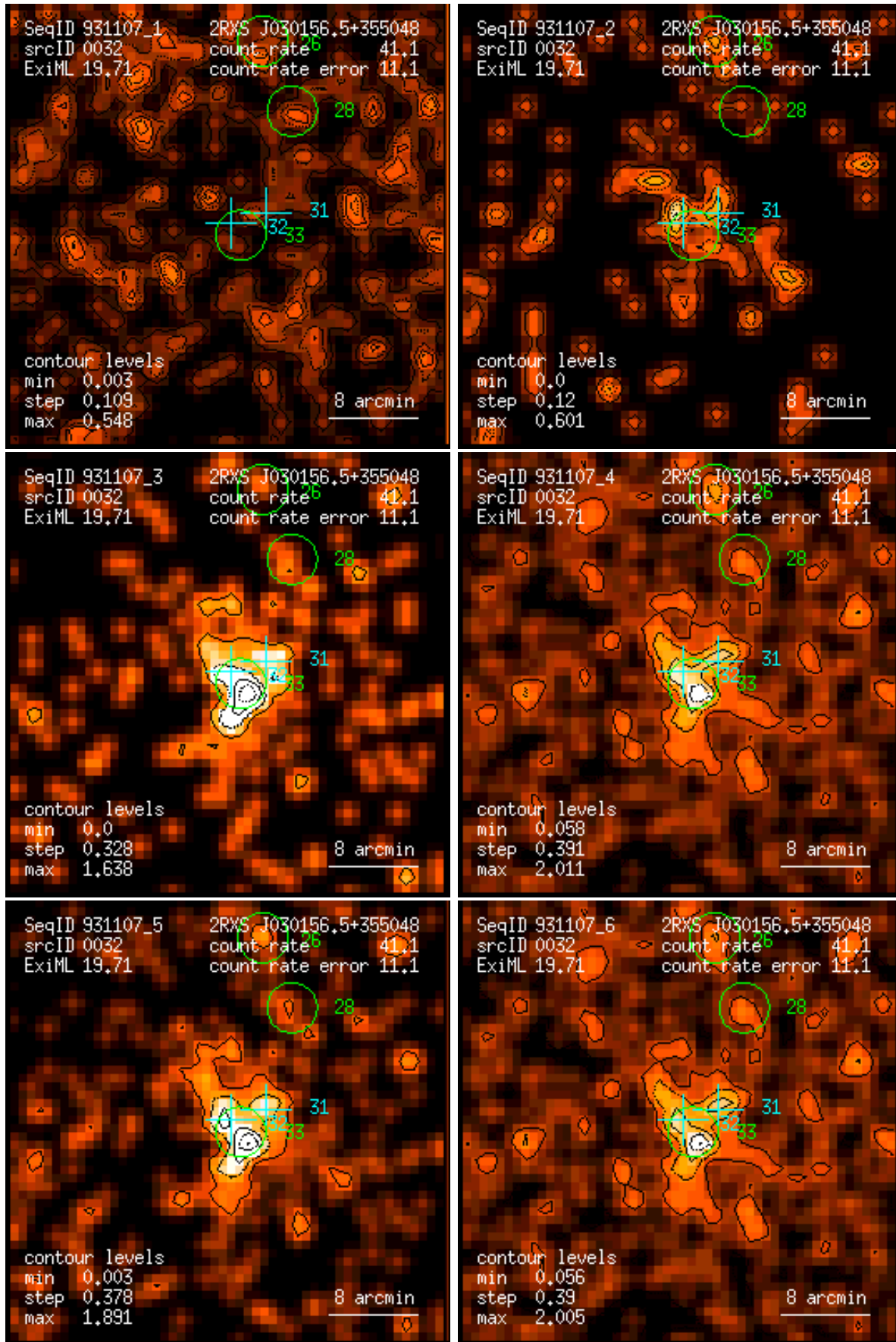
Figure 32: RASS 931107: detection 0032: band rate images, Gaussian filter: (1) PSPC channels 11 – 41, (2) 52 – 90, (3) 91 – 201, (4) 11 – 235, (5) 52 – 201, (6) 11 – 201. Broad band rates in counts/ks. Band rate contour levels in counts/ks/arcmin 2 .
